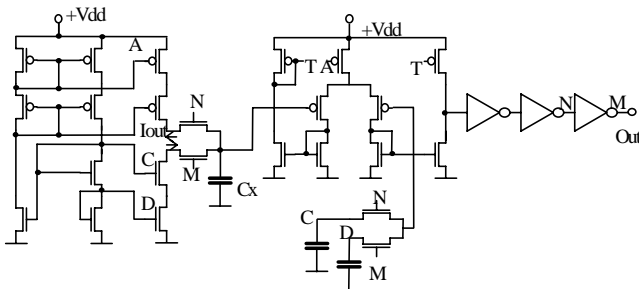
Figure 6 - Current-based temperature sensor with frequency-output
