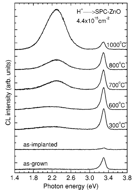
FIG. 9. Cathodoluminescence spectra measured for the H^+ -implanted ZnO after annealing at different temperatures.
