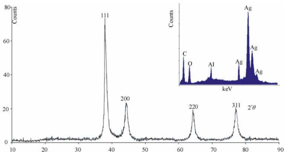
Figure 2. XRD pattern of crystalline AgNP synthesized using extracellular aqueous ethanolic carom seed extract. Inset fig. shows Energy dispersive x-ray spectrum EDAX of metallic biosynthesized AgNP.
