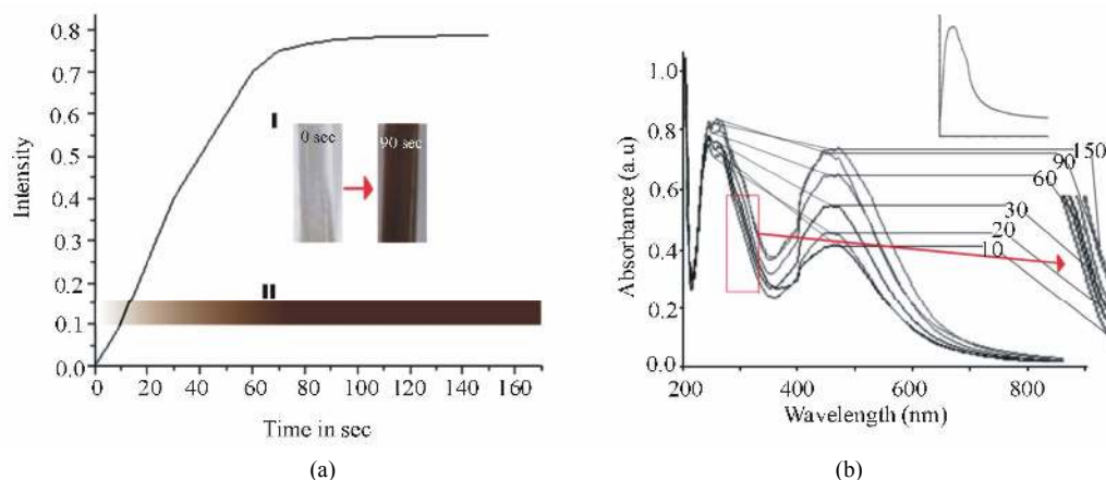
Figure 1. (a) Graph showing change in color intensity of the reaction mixture with respect to time. Inset: I. Initial and the final color of the reaction mixture containing aqueous 10^{-3} M \text{AgNO}_3 solution and aqueous ethanolic carom seed extract on microwave irradiation. II. Change in the color of the reaction mixture with time in sec. (b) UV-visible spectra of AgNP biosynthesis, absorbance recorded as a function of time. Projected and enlarged view of UV spectra is highlighted with an arrow line to show the stoppage of reaction at 90 sec. Inset: UV-vis spectrum of the extracellular carom seed extract.
