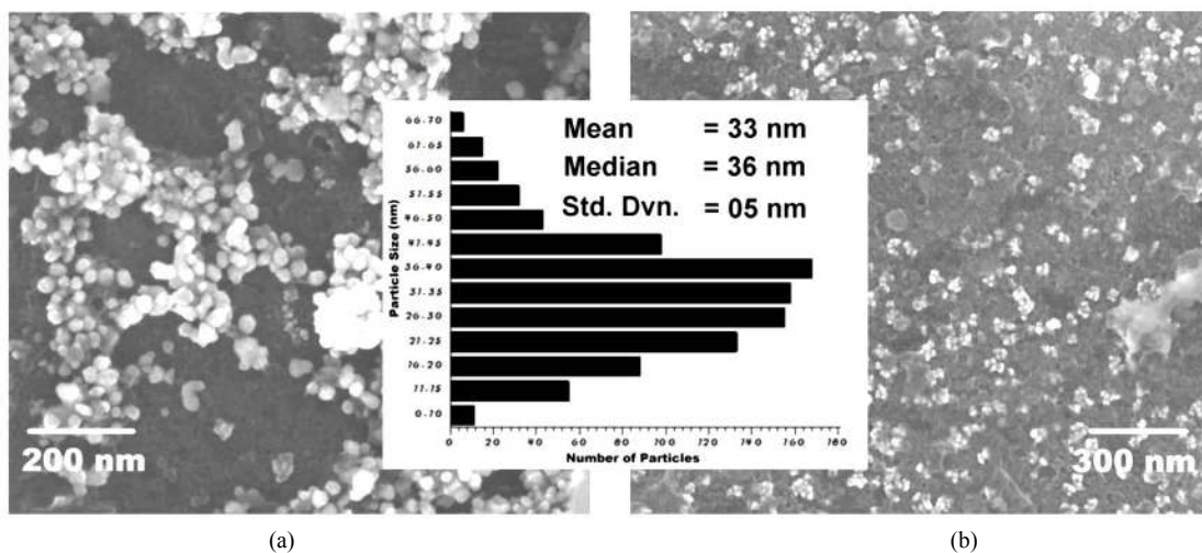
Figure 3. (a)& (b). FESEM images of synthesized AgNP in colloidal condition on different nanometric scale. Inset at the centre shows histogram indicating size distribution of AgNP.
