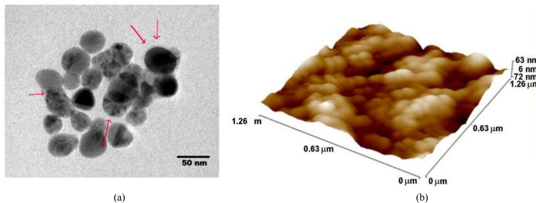
Figure 4. (a) TEM image of biosynthesized AgNP showing they are roughly spherical in shape. (b) Medium scale tapping mode AFM image of bio-functionalized AgNP adsorbed with organic layer.
