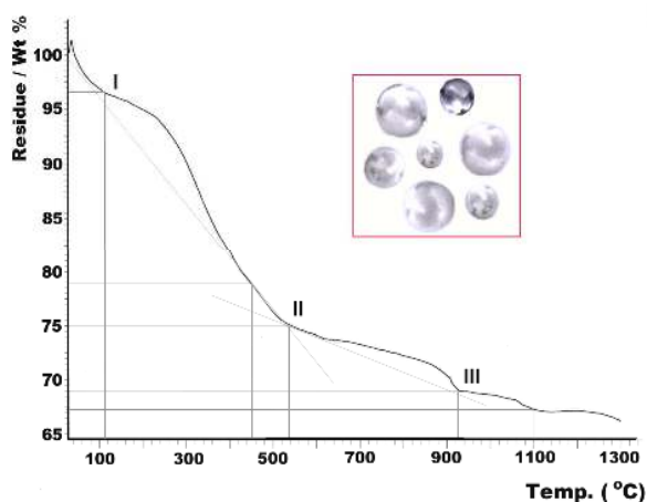
Figure 5. TGA graph showing the weight loss pattern of functional groups and other biological moieties adsorbed on the AgNP surface. Inset image shows bulk microstructures of pure silver as the residue left after cooling.
