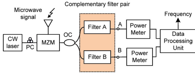
Fig. 1. Schematic of the proposed photonic microwave frequency measurement system. Mach-Zehnder modulator: MZM. Polarization controller: PC. Optical coupler: OC.
