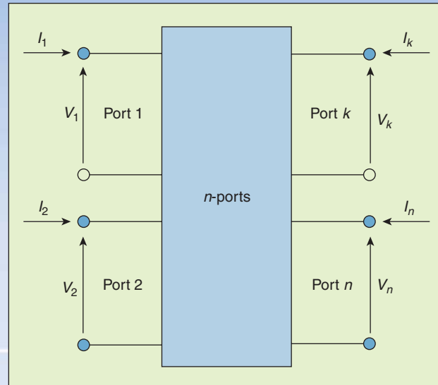
Fig. 1. System port voltage and current conventions adopted in S-Parameters calculations.
