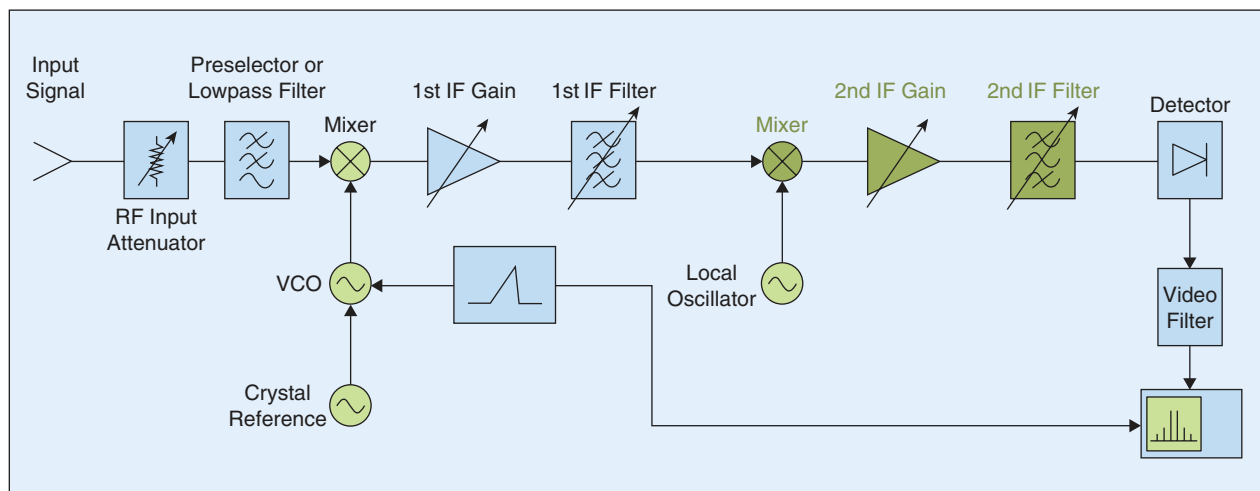
Fig. 6. Double IF conversion spectrum analyzer block scheme.
