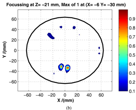
Fig. 8. 2D imaging results for experiment 3. (a) Results when CF = 1 (coherence quality weighting not applied). (b) Results after the CF weighting was applied.
