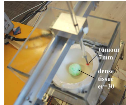
Fig. 3. Setup of the imaging experiment 1.
