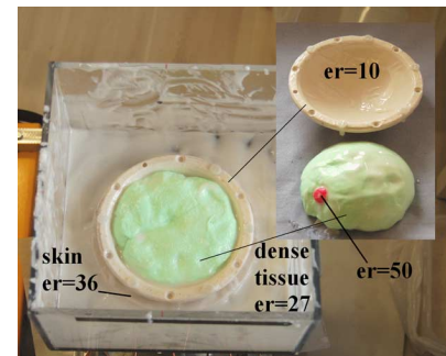
Fig. 4. Setup of the imaging experiment 2.
