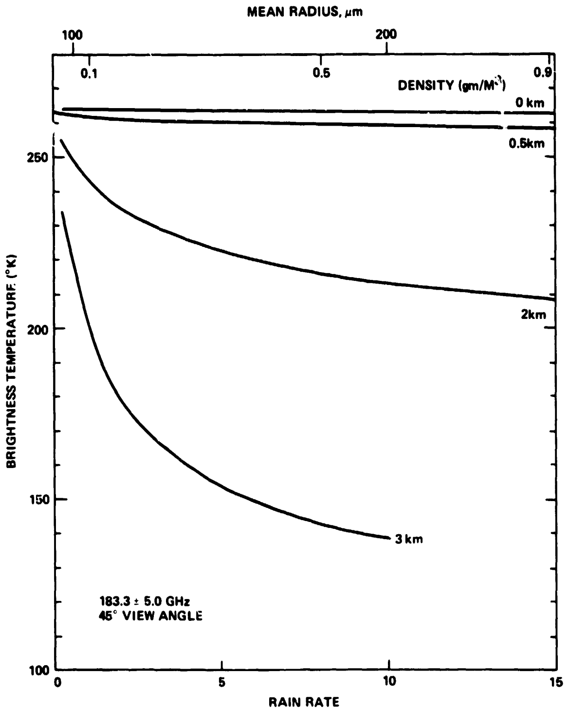
Figure 11. Brightness temperature calculations for 183 \pm 5.0 GHz. Numbers adjacent to curves indicate thickness of ice layer. The assumed freezing level is 5 km.
