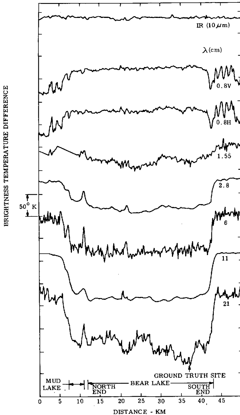
Figure 2. Multispectral data obtained over Bear Lake. The H and V refer to the horizontal and vertical channels of the 0.8 cm radiometer which viewed the surface at an angle of 45°. The remaining radiometers were nadir viewing. Average values for the brightness temperatures over the lake at each frequency are given in Table 2.
