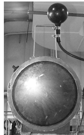
FIGURE 5. Photo of parametric sonar (bottom) and ITC 1001 transducer (top).
