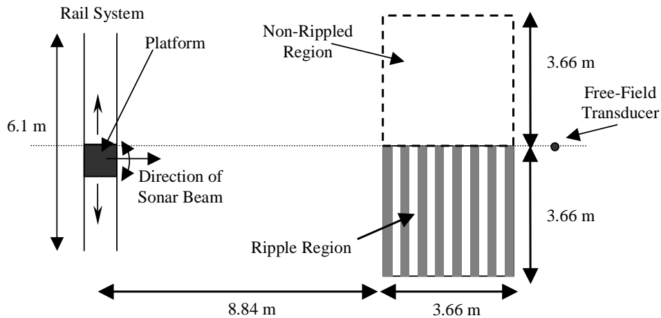
FIGURE 3. Scattering geometry.
