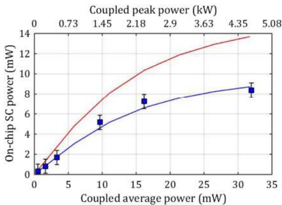
Fig. 5. On-chip SC power versus coupled average power measured for the 7 cm long waveguide (1) in TE at 4.0 \mu\text{m} (blue squares), simulated results for the 7 cm waveguide (blue line) and simulated results for a 2 cm long similar waveguide (red line).
