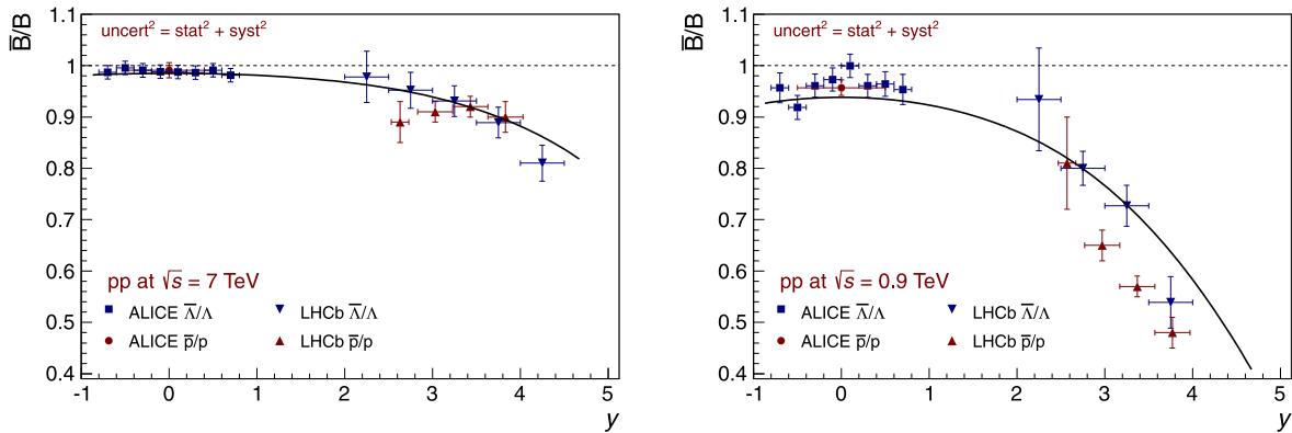
Fig. 17 \bar{p}/p and \bar{\Lambda}/\Lambda ratios as a function of rapidity at \sqrt{s} = 0.9 and 7 TeV. The parametrization with Eq. (4) (black line) is shown (Colour figure online)
