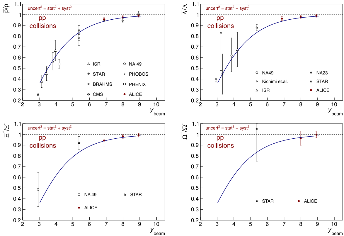
Fig. 16 Anti-baryon to baryon yields ratios as a function of beam rapidity for various baryons separately. The parametrization with Eq. (4) (blue line) is shown. The red points show the ALICE measurements (Colour figure online)
