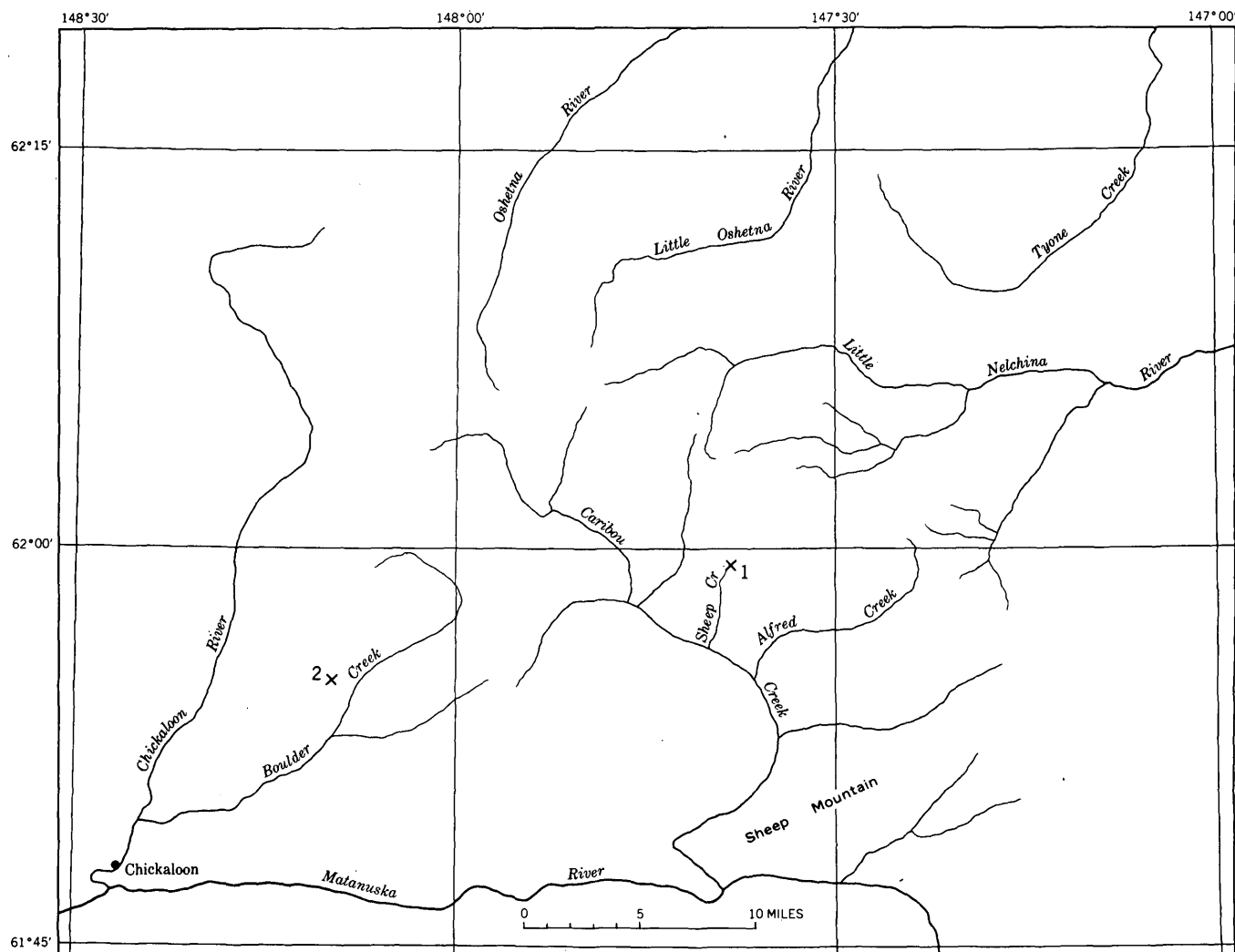
FIGURE 2.—Index map showing occurrences of upper Bajocian (Jurassic) fossils in the Talkeetna Mountains, Alaska. (Numbers on map refer to those given in the locality list (table 2) and in the distribution table.)
