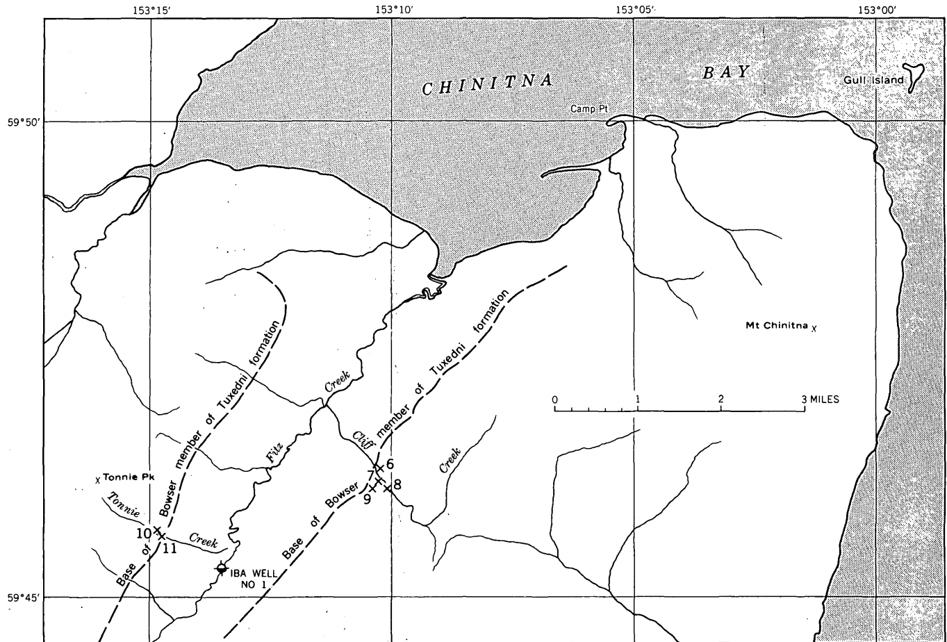
FIGURE 4.—Index map showing occurrences of upper Bajocian (Jurassic) fossils in the northern part of the Iniskin Peninsula. (Numbers on map refer to those given in the locality list (table 2) and in the distribution table.)
