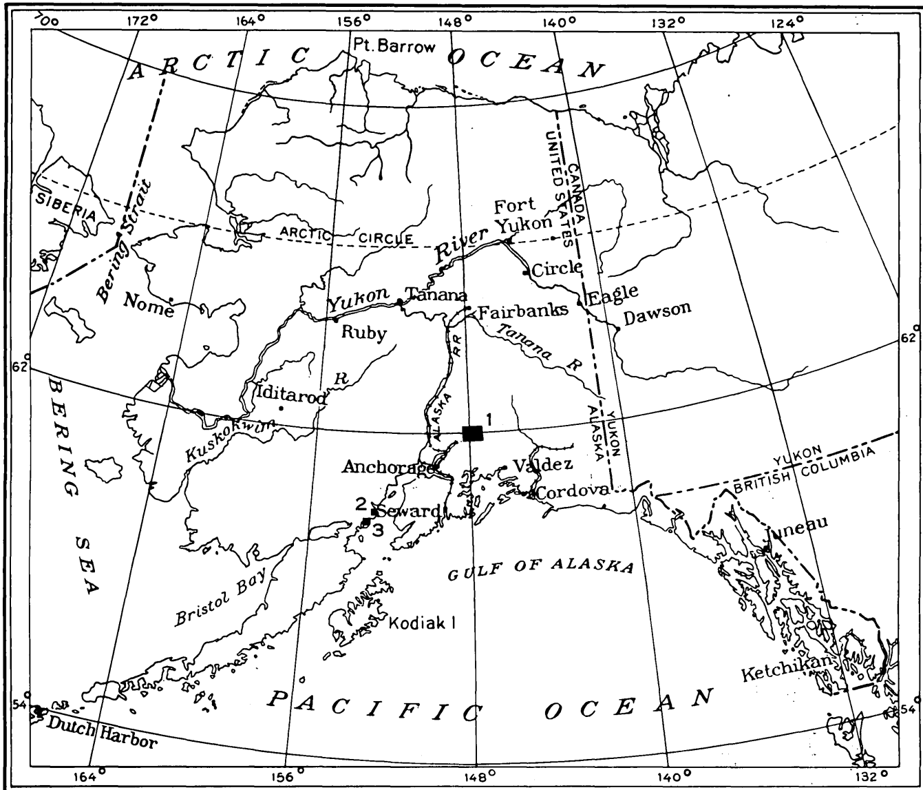
FIGURE 1.—Index map showing the principal areas of upper Bajocian (Jurassic) rocks in the Cook Inlet region, Alaska. (1) Eastern part of the Talkeetna Mountains; (2) Tuxedni Bay area; (3) northern part of the Iniskin Peninsula.
