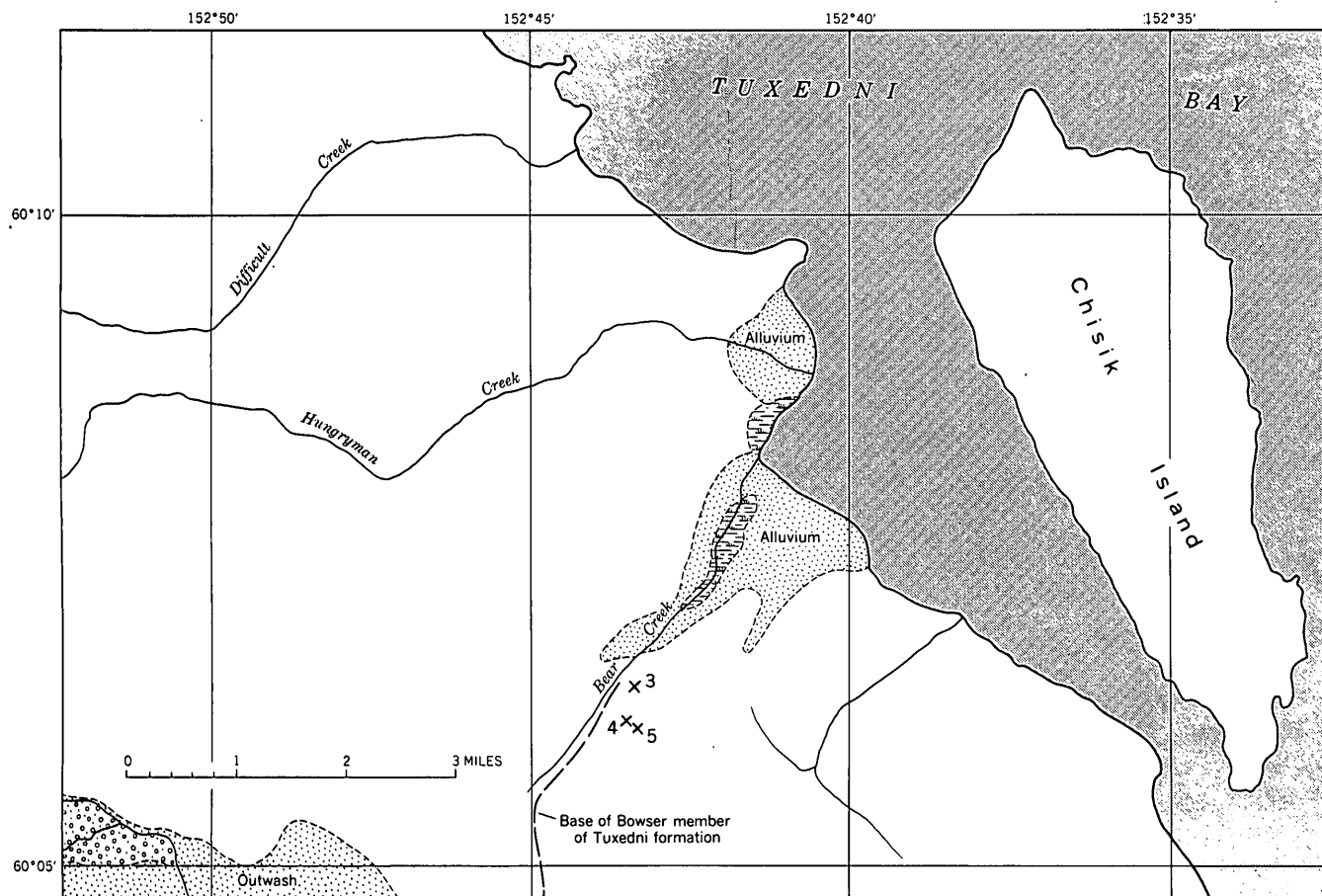
FIGURE 3.—Index map showing occurrences of upper Bajocian (Jurassic) fossils in the Tuxedni Bay area, Alaska. (Numbers on map refer to those given in the locality list (table 2) and in the distribution table.)
