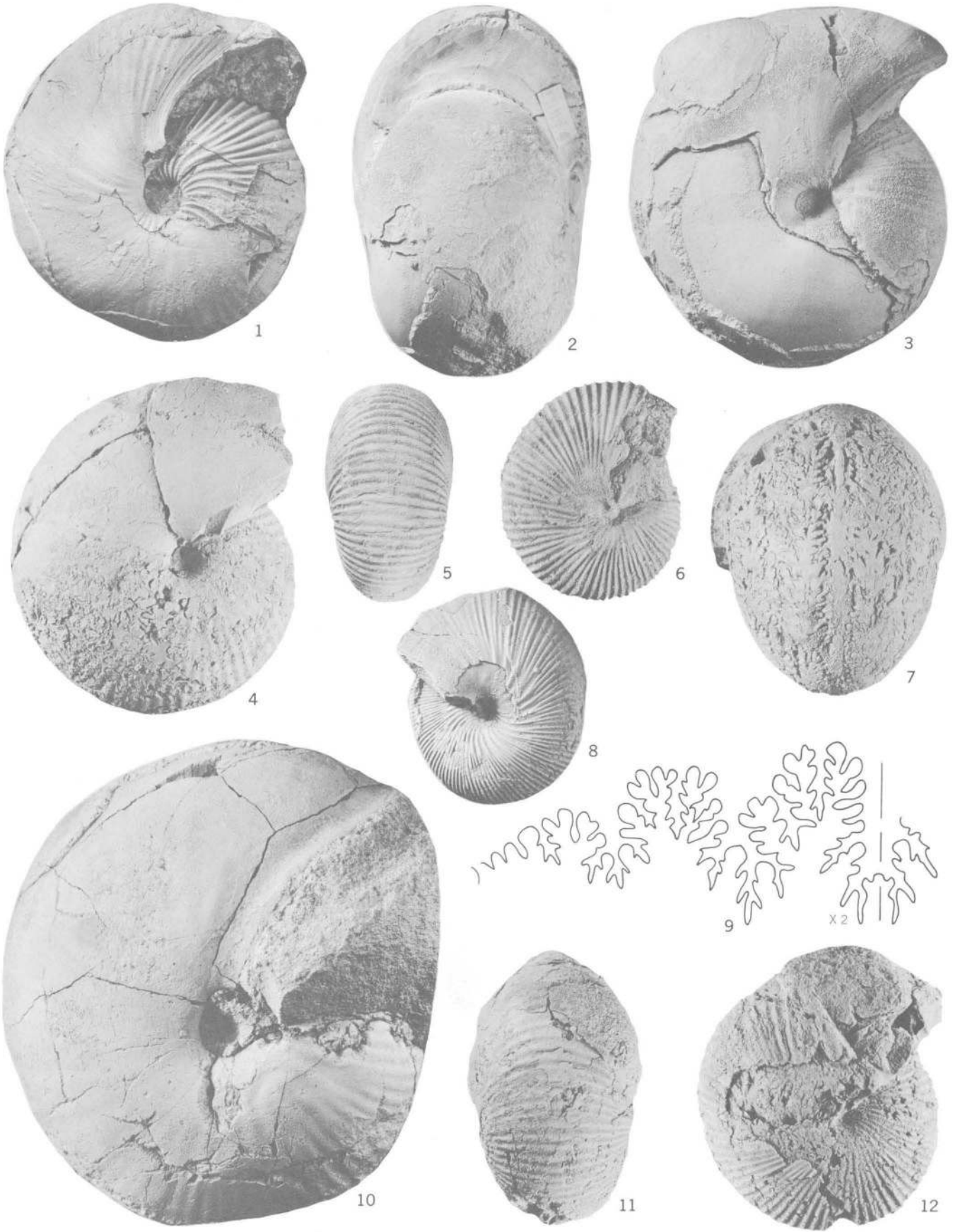
MEGASPHAEROCERAS
