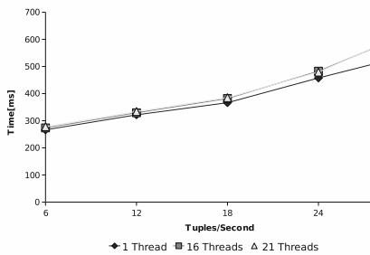
Fig. 10. Behaviour of PSA as the number of tuples/sec increases
