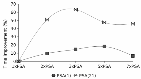
Fig. 11. Effect of the increase of number of PSA operators
