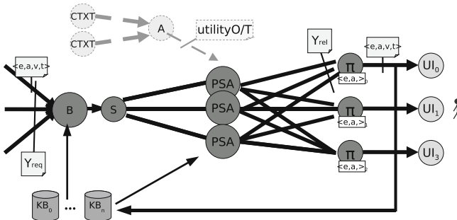
Fig. 8. Disclosure control
