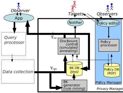
Fig. 6. PrivacyManager
