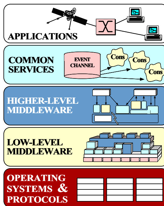
Figure 1: Layers of Middleware
