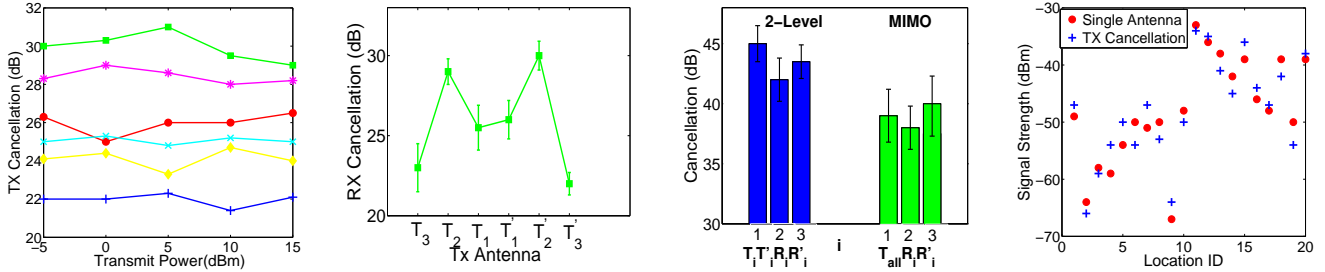
Figure 7: (a) Tx cancellation, (b) Rx cancellation, (c) 2-Level and MIMO cancellation; (d) Impact in far-field.
