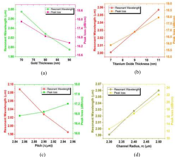
FIGURE 11. Resonant wavelength and corresponding loss as a function of (a) gold thickness, (b) TiO 2 thickness, (c) pitch and (d) channel radius.
