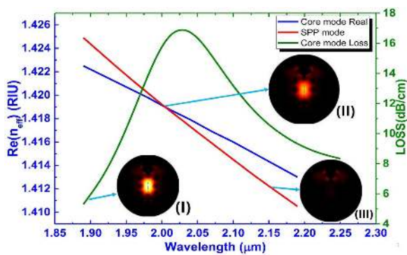
FIGURE 3. The real part of the effective index of the core mode (blue), SPP mode (red) and confinement loss of the core mode (green) with respect to wavelength alterations.
