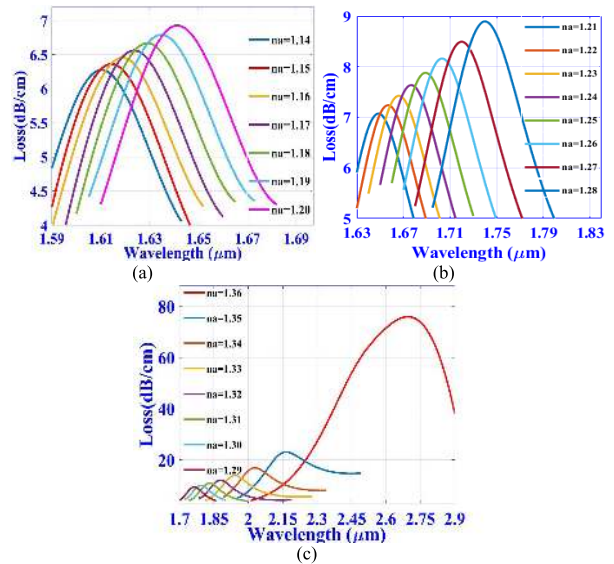
FIGURE 4. Loss curves for analyte refractive index variations (a) 1.14-1.20 (b) 1.21-1.28 and (c) 1.29-1.36.
