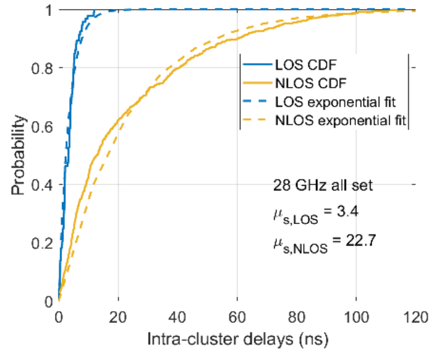
Fig. 7. Intra-cluster delays for 28 GHz LOS and NLOS all set.
