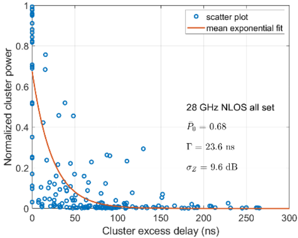
Fig. 8. Normalized cluster powers for 28 GHz NLOS all set.
