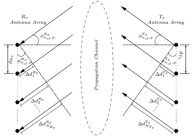
Figure 28. Outgoing and incoming signal rays of the p -th ray in the n_{cl} -th cluster at both T_x and R_x ULA antennas. Both arrays have separation distances d_{T_x}^{n_{cl},p} and d_{R_x}^{n_{cl},p} and corresponding departing and arriving angles \phi_{n_{cl},p}^{T_x} and \phi_{n_{cl},p}^{R_x} . The distance differences \Delta d between rays of the same ULA possess a specific progressive phase difference according to the antenna element position.
