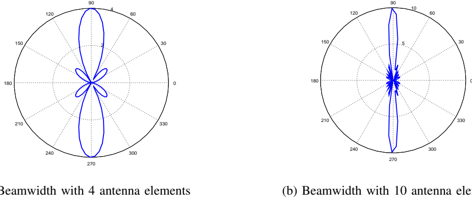
Figure 33. Polar plots representing the beamwidth of 4 and 10 antenna elements.
