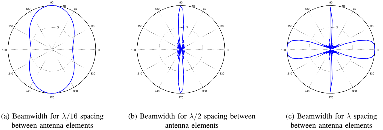
Figure 34. Polar plots representing the beam patterns at \lambda/16 , \lambda/2 , and \lambda spacing between antenna elements.
