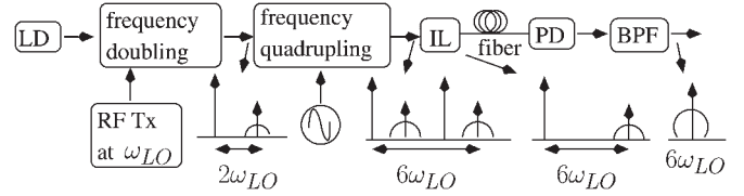
Fig. 35. Frequency six-tupling.
