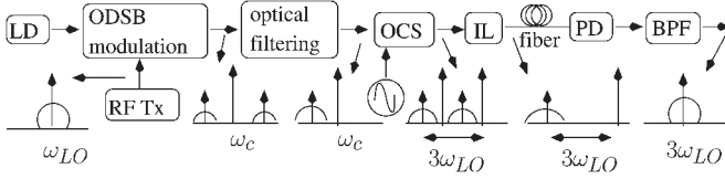
Fig. 31. Frequency tripling.
