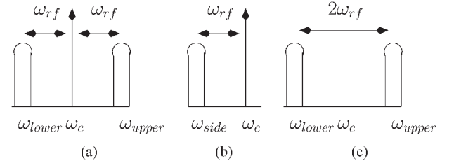
Fig. 15. Optical modulation formats. (a) Optical Double Side Band (ODSB) signal. (b) Optical Single Side Band (OSSB) signal. (c) Optical Carrier Suppression (OCS) signal.
