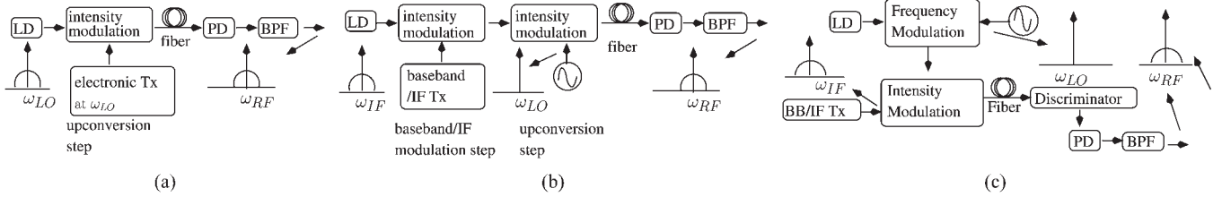
Fig. 24. N-tupling architectures (BB—Baseband; IF—Intermediate Frequency). (a) One-Step optical upconversion. (b) Two-Step optical upconversion. (c) Optical Frequency Multiplication (OFM).
