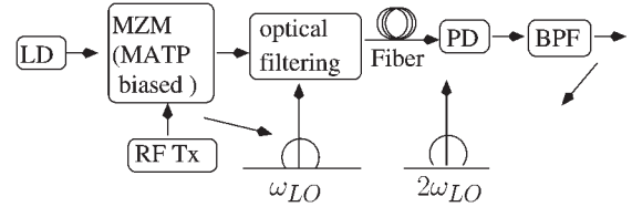
Fig. 29. Frequency doubling using Maximum Transmission Point (MATP) biasing.
