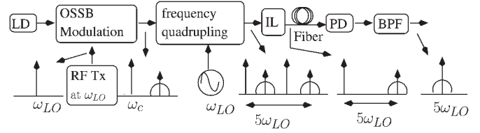
Fig. 34. Frequency quintupling.
