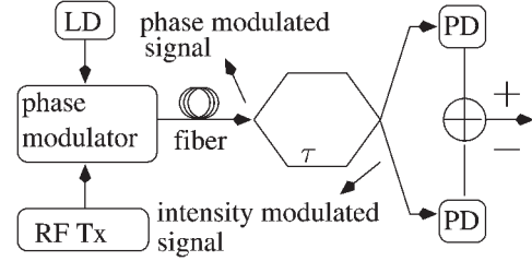
Fig. 18. Phase modulation using Mach-Zehnder delay Interferometer (MZI).
