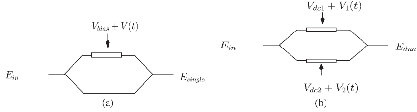
Fig. 7. Mach-Zehnder Modulator (MZM) external modulators. (a) Single drive MZM. (b) Dual drive MZM.
