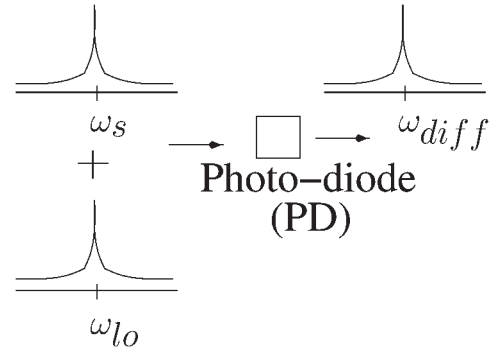
Fig. 12. Heterodyne photo-detection.
