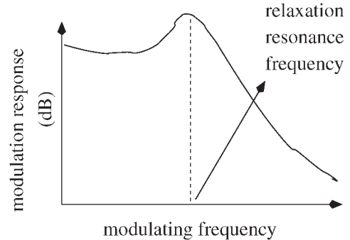
Fig. 6. Modulation bandwidth of the laser.
