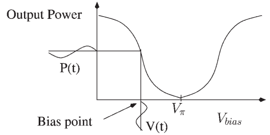
Fig. 8. Mach-Zehnder Modulator (MZM) transmittance.
