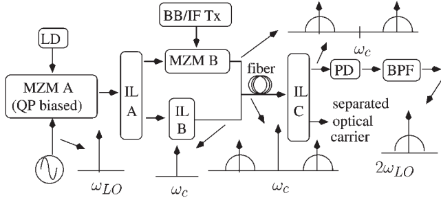
Fig. 30. Frequency doubling using quadrature biasing (IL-Interleaver).
