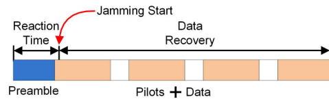
Fig. 5: Extended frame structure
