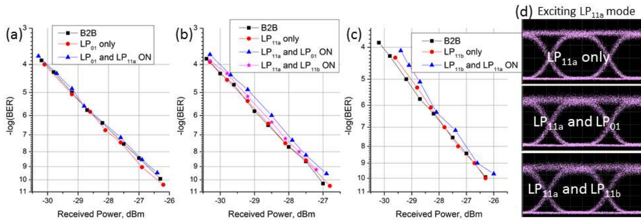
Fig. 2: BER curves for the various modes LP 01 (a), LP 11a (b) and LP 11b (c) with and without the other modes on, including back-to back curves. (d) Examples of eye diagrams of the signal transmitted in the LP 11a mode with and without the other signals transmitted in the LP 01 and LP 11b modes.
