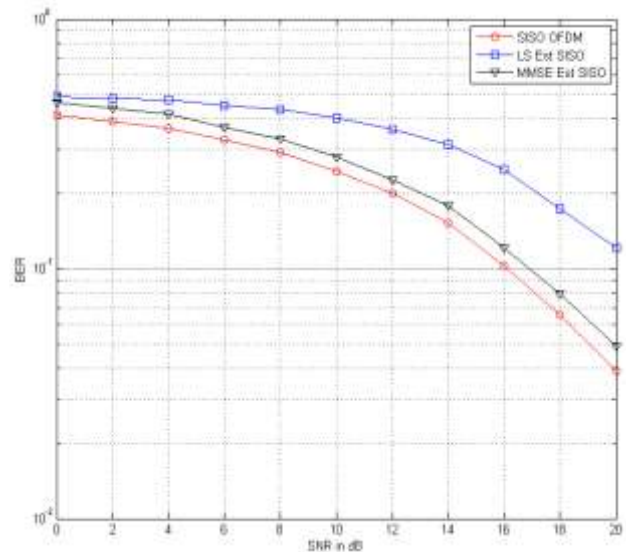
Figure 9. BER plot for comb type SISO OFDM with LS/MMSE Estimators
