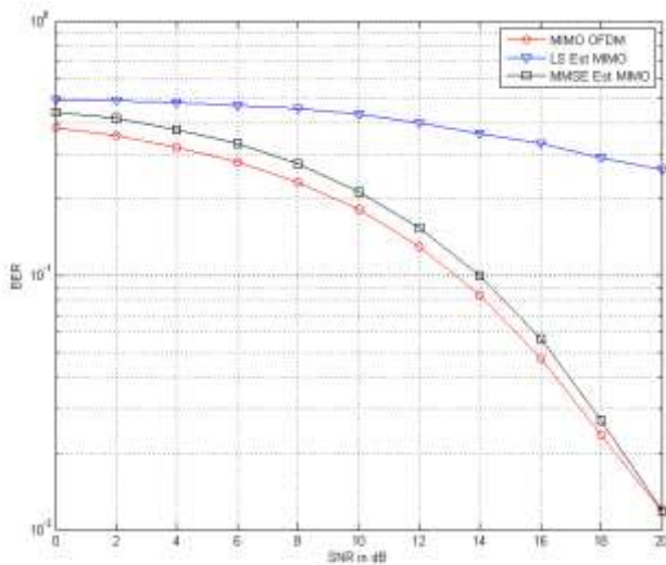
Figure 10. BER plot for comb type MIMO OFDM with LS/MMSE Estimators
