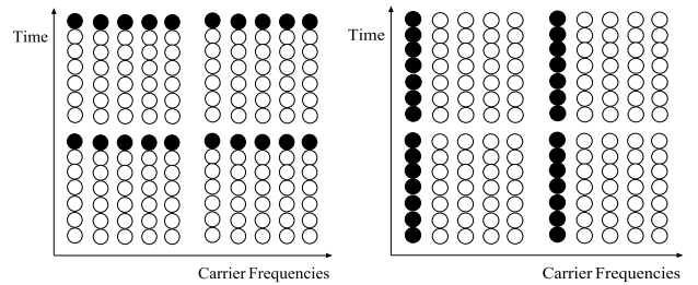
Figure 3.1. Block Pilot
