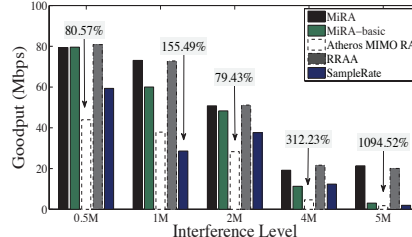
Figure 12: Goodput in hidden terminal.
