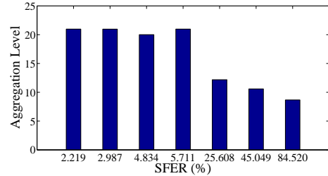
Figure 3: SFER vs. aggregation level.
