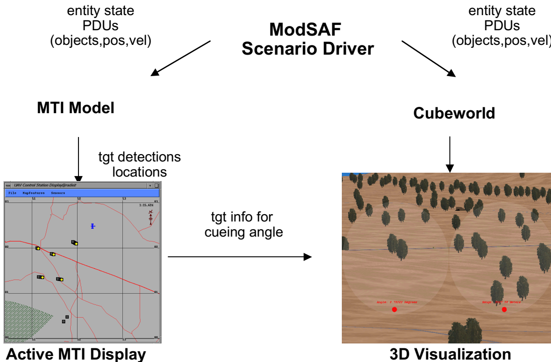
Figure 2-1: M2MTI/APLA Simulation Architecture
