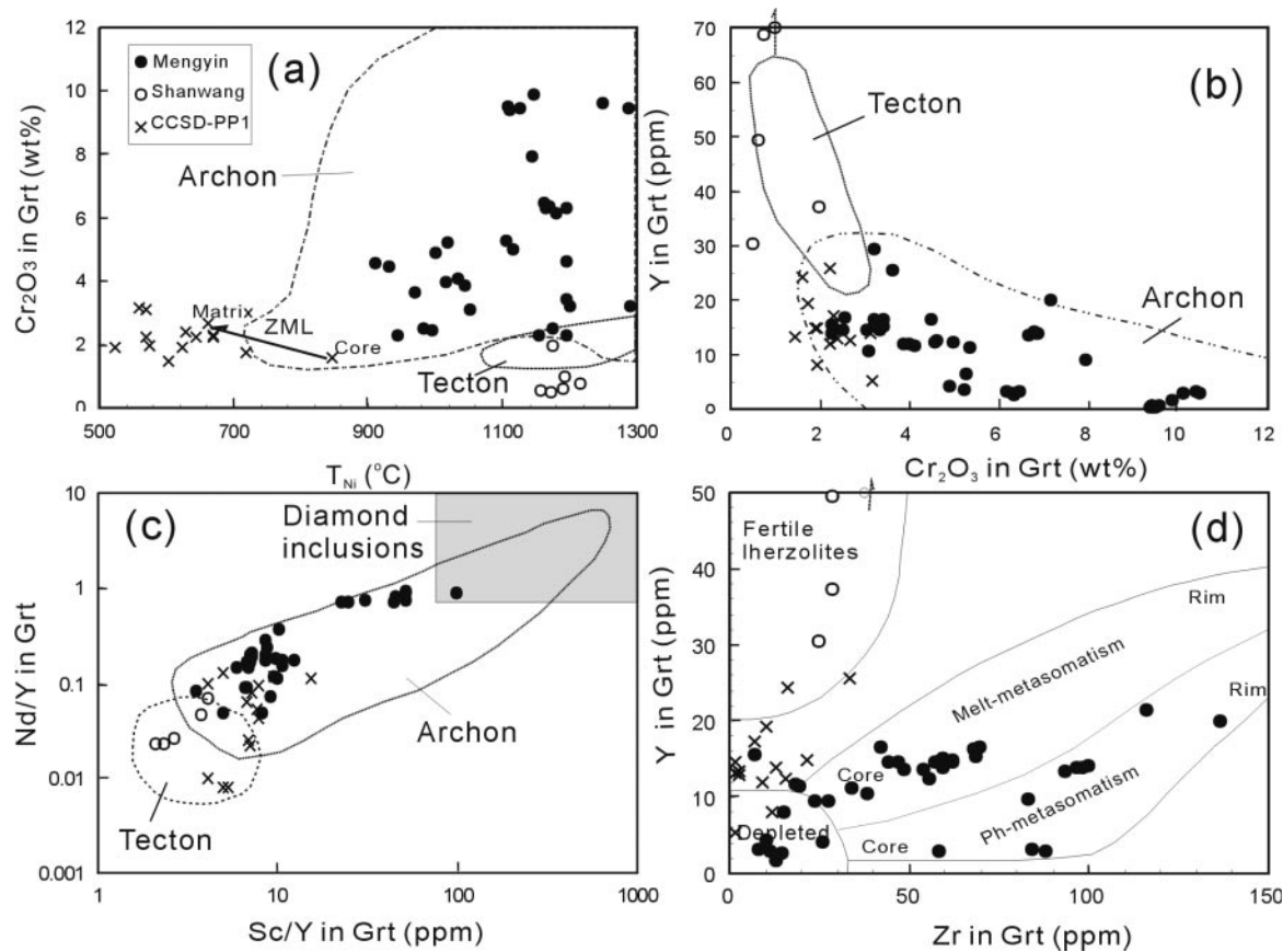
Fig. 10. \text{Cr}_2\text{O}_3 in garnet vs T_{\text{Ni}} (a); \text{Cr}_2\text{O}_3 vs Y in garnet; (c) Nd/Y vs Sc/Y in garnet; (d) Zr vs Y in garnet. Fields for diamond-inclusion garnets, and garnets from Archon and Tecton, after Griffin et al. (1998a, 1998b, 1999a, 1999b). Fields showing trace-element signatures of garnets from depleted harzburgite and fertile lherzolite, and different metasomatic styles are from Griffin & Ryan (1995). Melt-related metasomatism is typical of high- T sheared lherzolite xenoliths in kimberlites; phlogopite-related metasomatism is seen in garnets from shallower phlogopite-rich lherzolites in kimberlites. Core–rim zoning with increase in Zr is characteristic of both metasomatic styles (Griffin & Ryan, 1995). Data for sample ZML from Zheng et al. (2005a).
