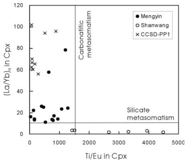
Fig. 11. Ti/Eu vs (\text{La}/\text{Yb})_{\text{N}} (chondrite-normalized) of Cpx in the CCSD-PP1, Mengyin and Shanwang peridotites. Signatures of silicate and carbonatitic metasomatism are modified after Coltorti et al. (1999).
