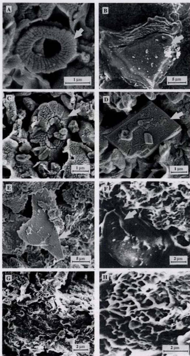
FIG. 7. Top 4 photos show the scanning electron micrographs (SEM) of the calcite-rich bentonite. (A) = BAL-1, (B) = BAL-2, (C) = BAL-5, and (D) = BAL-6. Bottom 4 photos show the scanning electron micrographs (SEM) of the cristobalite-rich bentonite. (E) = BAL-3, (F) = BAL-4, (G) = BAL-7, and (H) = BAL-9. Arrow markers indicate microfossils in A and C, volcanic glass relics in B, E and F, and crystal in D.
