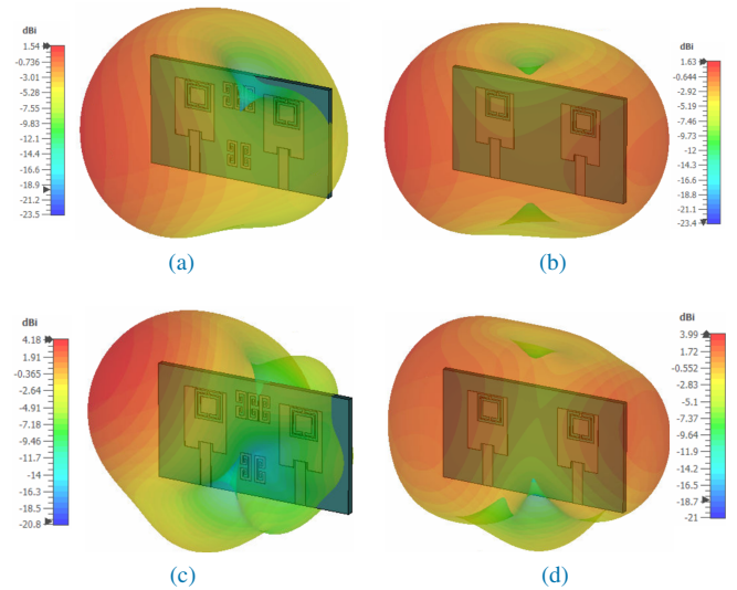
FIGURE 14: 3D radiation patterns of the proposed antennas: (a) 2.4 GHz with MTMs, (b) 2.4 GHz without MTMs, (c) 5.8 GHz with MTMs, (d) 5.8 GHz without MTMs.
