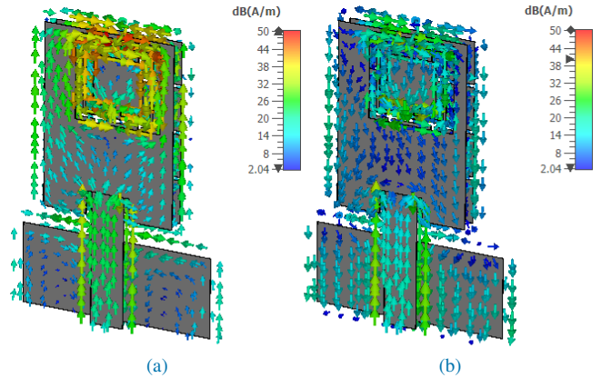
FIGURE 5: Snapshot of the antenna's current distribution at (a) 2.45 GHz and (b) 5.8 GHz.
