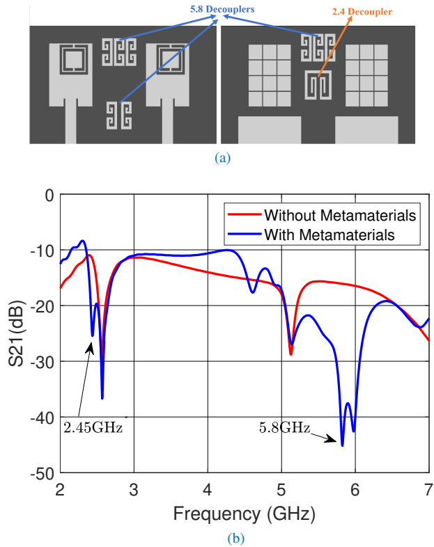
FIGURE 10: (a) Antennas using decoupling structure and (b) coupling coefficient S_{21} derived through simulations versus frequency.
