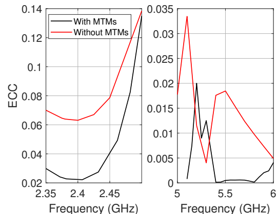
FIGURE 16: Envelope correlation coefficient (ECC) versus frequency at 2.35-2.5 GHz (lower band) and 5-6 GHz (higher band)
