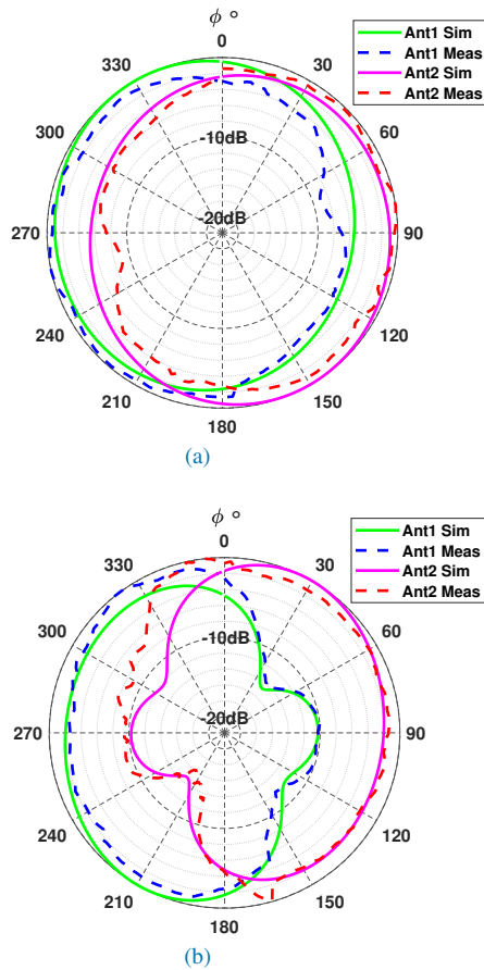
FIGURE 13: Normalized, H-plane, Co-Pol. radiation patterns of the two antennas at (a) 2.4 GHz and (b) 5.8 GHz. Both the simulations and measurements refer to the case with extended ground planes.
