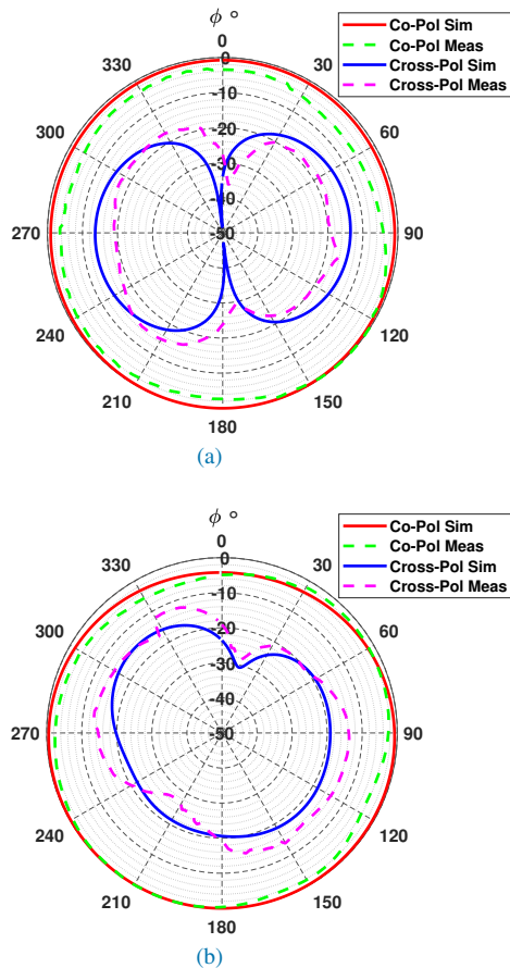
FIGURE 7: Normalized H-plane radiation patterns of the proposed small antenna at (a) 2.4 GHz and (b) 5.8 GHz. The simulations do not include the ground plane extension that was utilized during the measurements.
