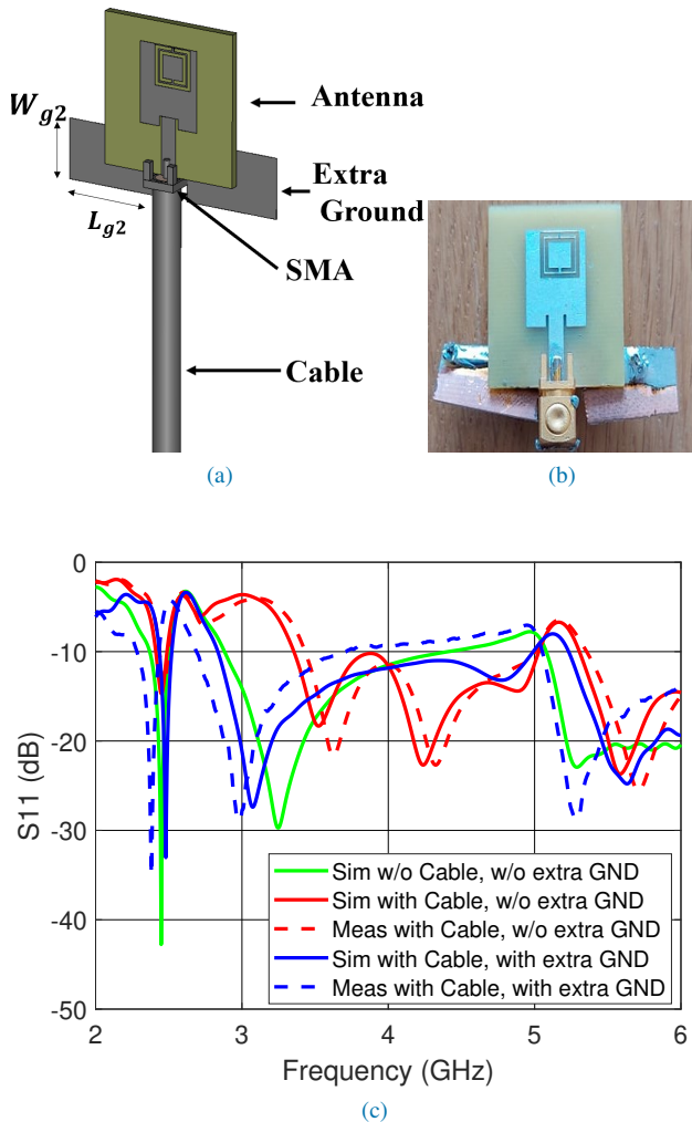
FIGURE 6: (a) Simulation of the antenna with the attached cable and extended ground plane in order to model the measurement setup, (b) fabricated prototype with extra ground plane and connector and (c) simulated and measured reflection coefficient S_{11} versus frequency for different configurations of the antenna. The cable that is considered here has a characteristic impedance of 50 \Omega and a length of 150 mm.
