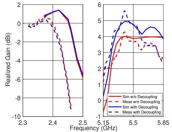
FIGURE 15: Measured realized gain of the proposed antennas with and without metamaterial decoupling at 2.32-2.5 GHz and 5.15-5.85 GHz frequency bands. Both the simulations and measurements refer to the case with extended ground planes. The antenna resonates around 2.37 GHz in practice and therefore the realized gain was measured from 2.32 to 2.45 GHz.
