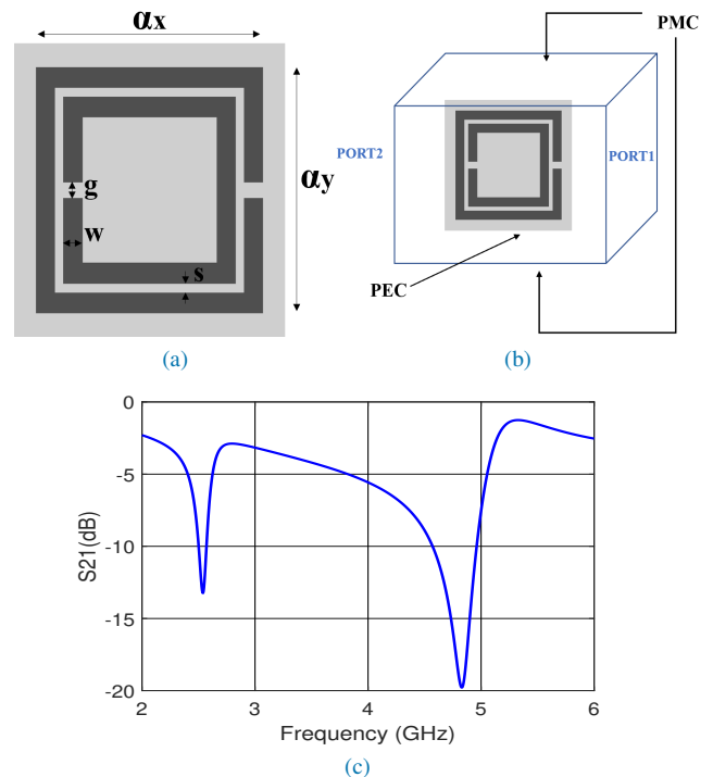
FIGURE 2: (a) The geometry of a CSRR unit cell, (b) its simulation setup and (c) the optimized transmission coefficient S_{21} . Light grey depicts metallization. The CSRR parameters in millimeters are: \alpha_x = 8.3, \alpha_y = 8.3, w = 0.7, s = 0.3 and g = 0.5 .
