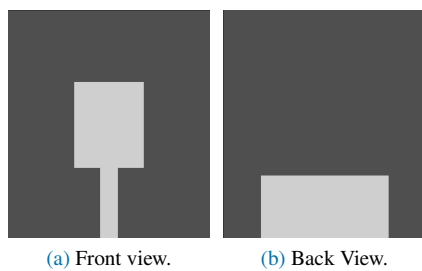
FIGURE 1: Unloaded, printed monopole antenna fed by a microstrip line.
