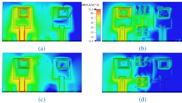
FIGURE 11: Electromagnetic power flow within the structure when port 1 (left) is excited and port 2(right) is connected to 50 \Omega : (a) 2.45 GHz without MTMs, (b) 2.45 GHz with MTMs, (c) 5.8 GHz without MTMs, (d) 5.8 GHz with MTMs.
