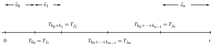
Fig. 1. How the interval [0, t] is split up into subintervals.
