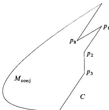
FIGURE 7. The conjugate of a fundamental piece for the higher genus prismoids.
