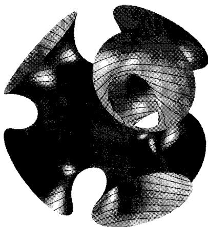
(3) \mathcal{P}_0(2n, \theta) for n=3 and \theta=45 degrees
