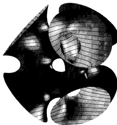
(4) \mathcal{P}_{n-1}(2n, \theta) for n=3 and \theta=45 degrees
