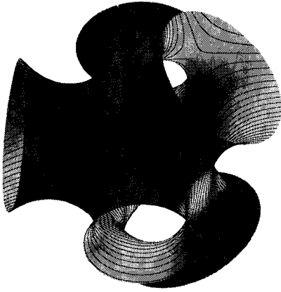
(1) \mathcal{JMV}_0(n+2, w) for n=3 and w \approx 5/2
