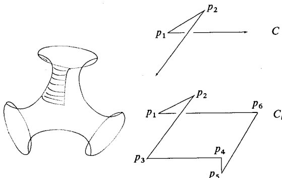
FIGURE 4. A fundamental piece of the Jorge-Meeks surface, boundary contour C of the conjugate of the fundamental piece, and the compact boundary contours C_i .
