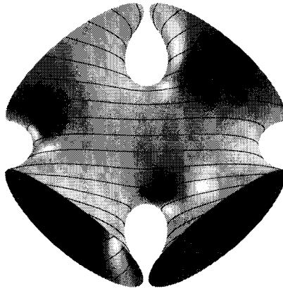
(3) \mathcal{AA}_0(2n, \theta) for n=2 and \theta=30 degrees
