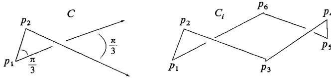
FIGURE 5. The boundary contour C of the conjugate of a fundamental piece of the tetroid, and the compact boundary contours C_i .
