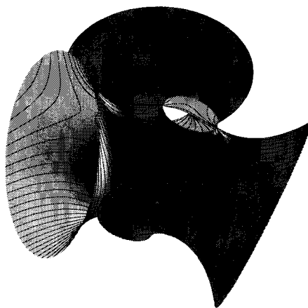
(2) Jorge-Meeks n -oid fence with n=3
