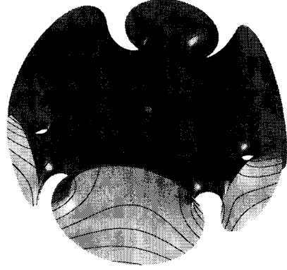
(2) \mathcal{AW}_0(2n, w) for n=3 and w \approx 5/2
