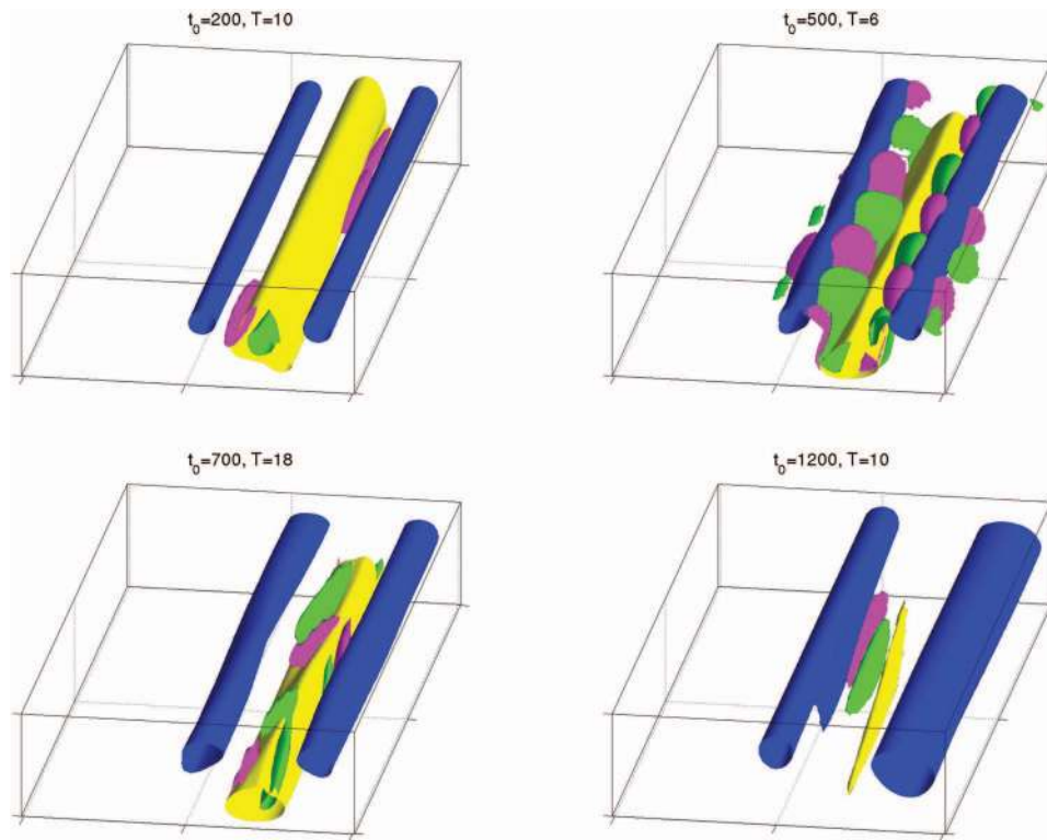
FIG. 14. Wall-normal velocity isosurface |u_y| = C_y \max u_y of the Lyapunov perturbation (pink: u_y > 0 , green: u_y < 0 ). Streamwise perturbation velocity isosurface |u_x| = C_x \max u_x of the edge trajectory (yellow: u_x > 0 , blue: u_x < 0 ). From left to right, top to bottom: (a) t_0 = 200 , T = 10 ; (b) t_0 = 500 , T = 6 ; (c) t_0 = 700 , T = 18 ; and (d) t_0 = 1200 , T = 10 . Same isometric view as Fig. 4. C_x = 0.55 except for t_0 = 200 : C_x = 0.3 and t_0 = 1200 : C_x = 0.9 , C_y = 0.4 except for t_0 = 1200 where C_y = 0.7 .
