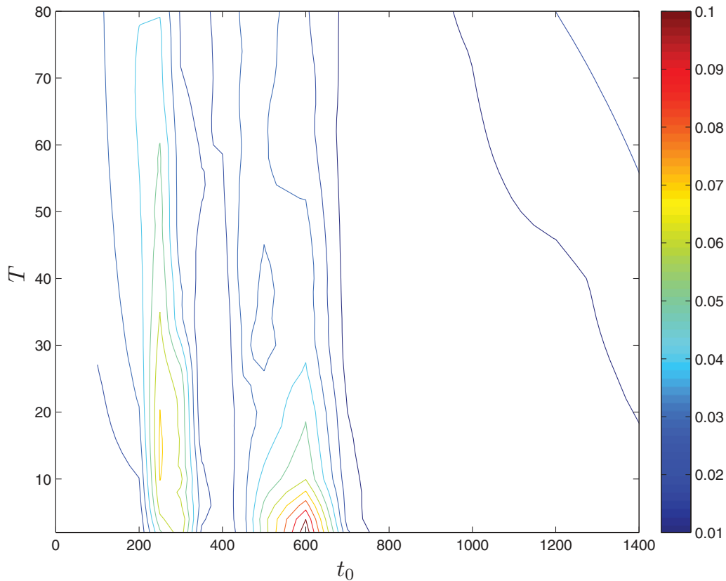
FIG. 12. Finite-time Lyapunov exponent \lambda^T(t_0) as function of t_0 and T along the edge trajectory.
