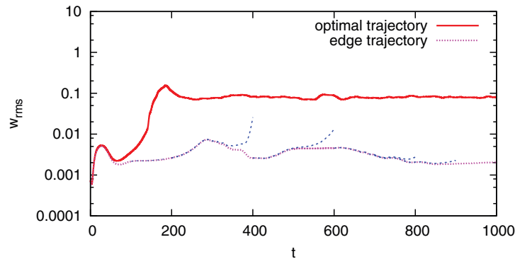
FIG. 11. w_{rms}(t) for the turbulent trajectory (solid/red) starting from the minimal seed, the edge trajectory (dotted/purple) starting from the rescaled minimal seed. Evolution of initially small deviations from the edge trajectory (dashed/blue).
