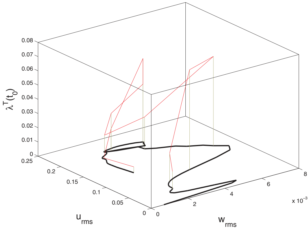
FIG. 13. Thin line (red): Finite-time Lyapunov exponent \lambda^T(t_0) as a function of u_{rms}(t_0) and w_{rms}(t_0) for T = 10 and t \leq 1000 . Thick line (black): Projection of the edge trajectory in the plane (u_{rms}, w_{rms}) .
