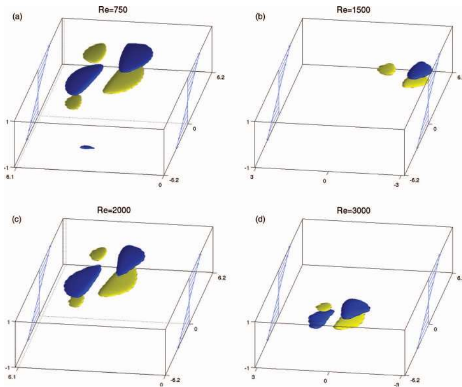
FIG. 4. Nonlinear optimal conditions for Re = 750, 1500, 2000, and 3000 . Iso-contours of the streamwise velocity perturbation u' corresponding to \pm 0.65 \max u_x . Blue arrows represent the base flow U_x = y .
