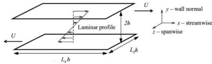
FIG. 2. Geometry and notations for plane Couette flow.
