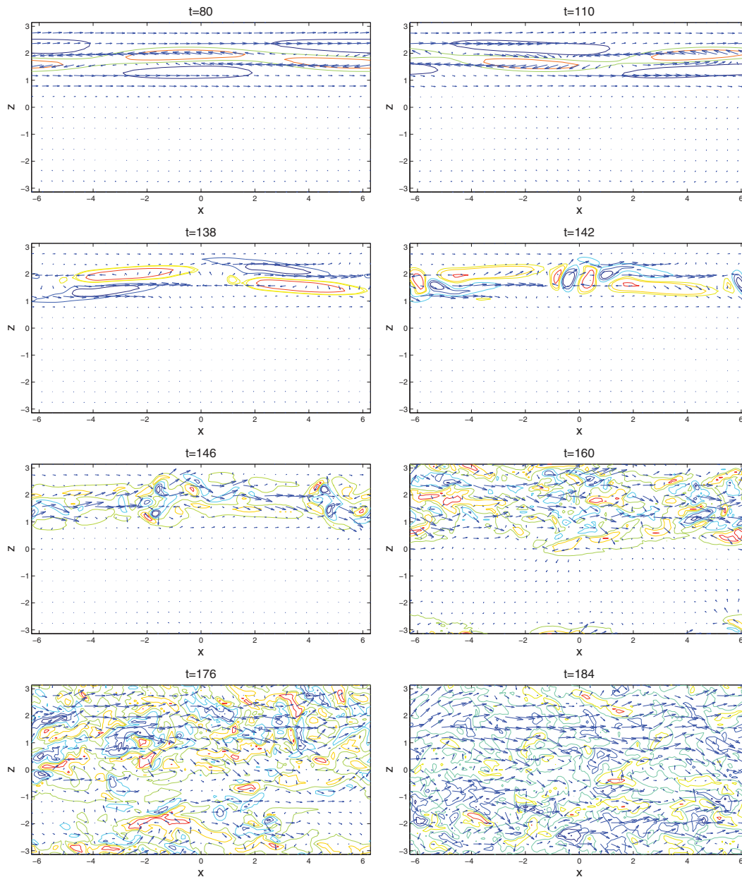
FIG. 10. Velocity field in the plane p_y: y = -0.5 . u_y : colours, (u_x, u_z) : arrows. Iso-contours of u_y normalised by their maximum, where \max u_y = 0.0055 ( t = 80 ), 0.0117 ( t = 110 ), 0.052 ( t = 138 ), 0.1023 ( t = 142 ), 0.2329 ( t = 146 ), 0.3333 ( t = 160 ), 0.3273 ( t = 176 ), and 0.5473 ( t = 184 ).
