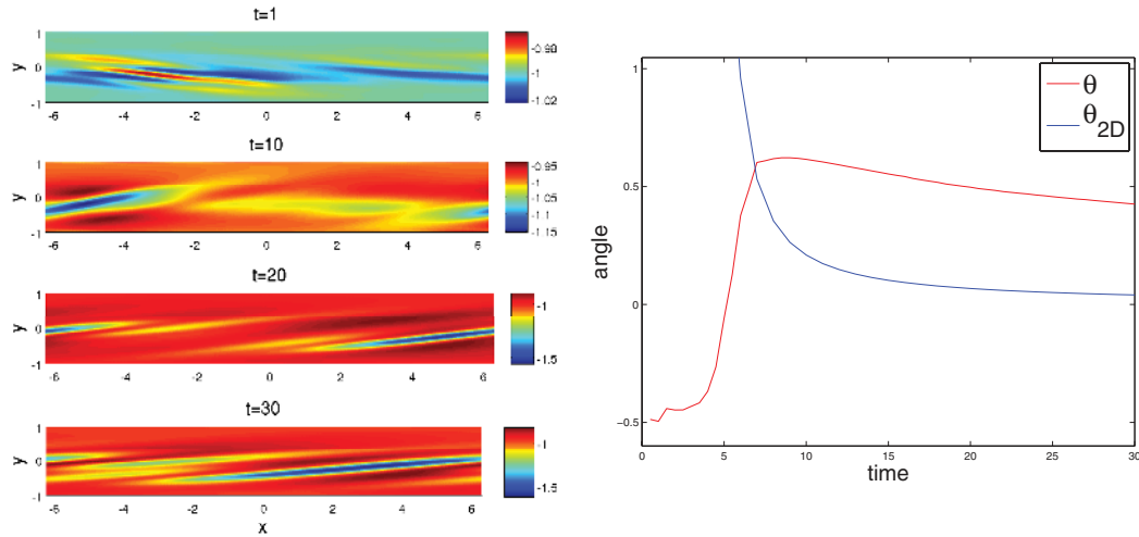
FIG. 7. Left: Spanwise vorticity \omega_z in the plane p_z : z = -\frac{\pi}{2} at times t = 1, 10, 20, and 30 . Right: Angle \theta computed using the second eigenvalue of the Hessian tensor of \omega_z at the minimum of \omega_z|_{p_z} vs. time. Comparison with theoretical two-dimensional angle \theta_{2D}(t) for a Kelvin wave solution.
