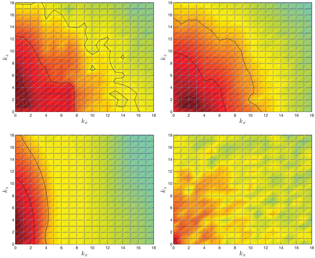
FIG. 5. Spectral distribution of kinetic energy \log e(k_x, k_z) normalised by its maximum, for the minimal seed for Re = 1500 at t = 0 , t = 10 , t = 100 , and t = 180 (from left to right and from top to bottom). The iso-contours correspond to E/\max(E) = 10^{-1} , 10^{-5} , and 10^{-10} .
