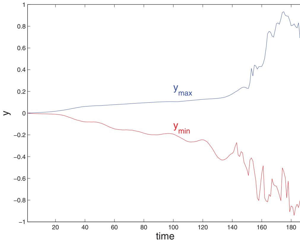
FIG. 9. Wall-normal positions of the maxima and minima of the iso-surface U_x + u_x = 0 vs. time.
