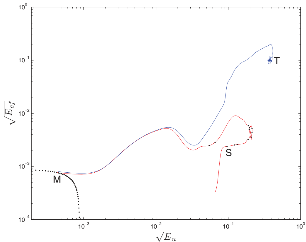
FIG. 15. (\sqrt{E_u}, \sqrt{E_{cf}}) projection of phase space with the nonlinear optimal trajectory (blue), the associated edge trajectory (red), and \epsilon_0 = E_c (black dots) for Re = 1500 . To be compared with Fig. 1.
