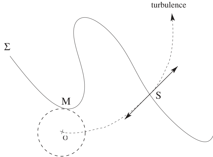
FIG. 1. Schematic view of the phase-space associated to the flow. O is the (stable) laminar state. \Sigma represents the laminar-turbulent boundary. The “edge state” S is the (unstable) asymptotical state on \Sigma . M is the minimal perturbation able to trigger transition to the turbulent state, i.e., the point on \Sigma closest to O in energy norm.
