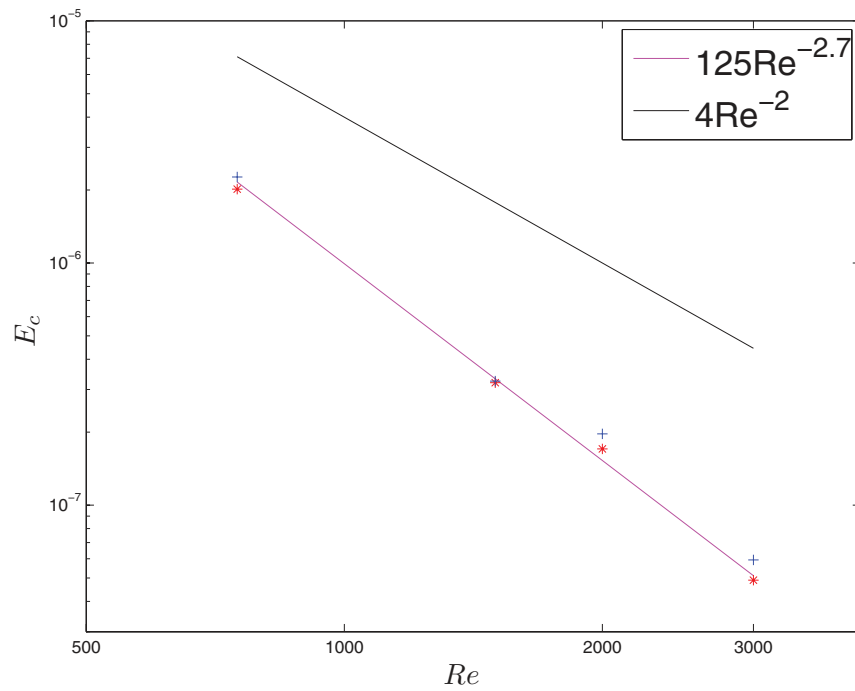
FIG. 3. Energy threshold E_c vs. Re for Re = 750, 1500, 2000, and 3000 . Stars represent the largest tested value of E_0 below which transition never occurs, while crosses represent the smallest tested value of E_0 for which transition occurs at least once. The fit 125Re^{-2.7} (pink) is compared to the fit 4Re^{-2} (black) obtained for the Oblique Wave scenario for the same computational box (data from Ref. 27).
