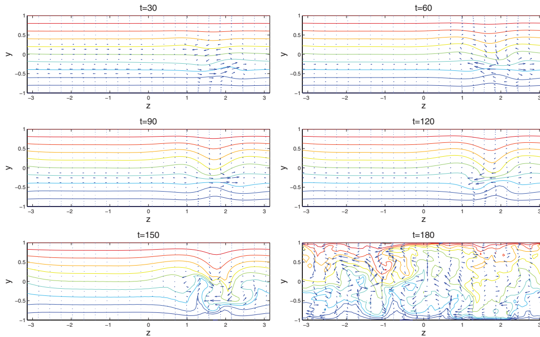
FIG. 8. Cross-sections of the velocity field in the plane p_x : x = 0 , for times t = 30, 60, 90, 120, 150 , and 180 . Contours: iso-levels of U_x + u_x ; arrows: (u_y, u_z) vectors.
