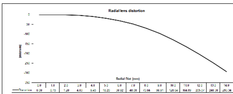
Figure 4. Radial distortion curve for one of the Nikon D80 cameras
