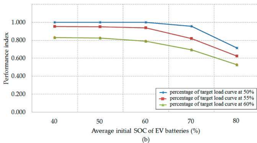
Figure 9. Performance Index under various scenarios: (a) peak load shaving and (b) load levelling.
