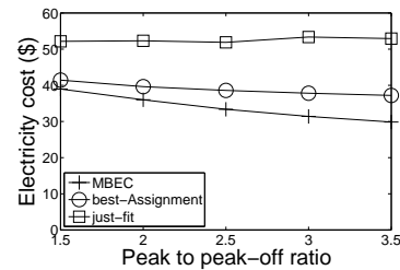
Figure 15: Electricity cost as against to peak to peak-off ratio.
