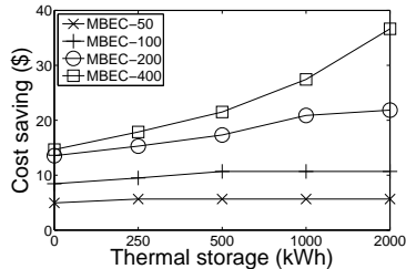
Figure 19: Electricity cost saving as against to thermal storage.
