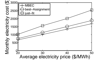
Figure 14: Monthly electricity cost as against to average electricity price.
