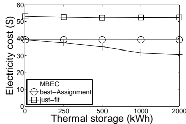
Figure 18: Electricity cost as against to thermal storage.
