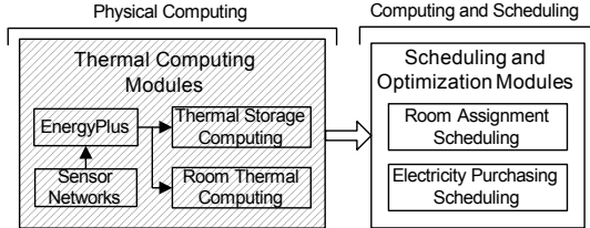
Figure 2: The framework of the thermal cost management system
