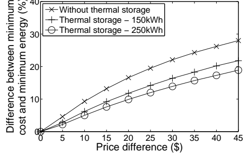
Figure 4: Difference between minimizing electricity and minimizing energy consumption as against to the price difference.
