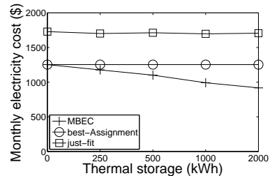
Figure 20: Monthly cost as against to thermal storage.
