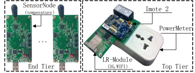
Figure 5: The Sensor System.
