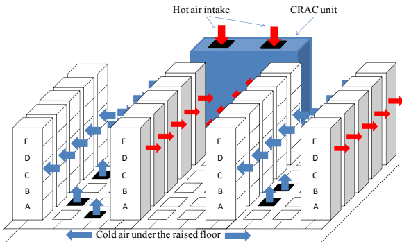
Figure 1. Hot-aisle/cold-aisle data center structure.
