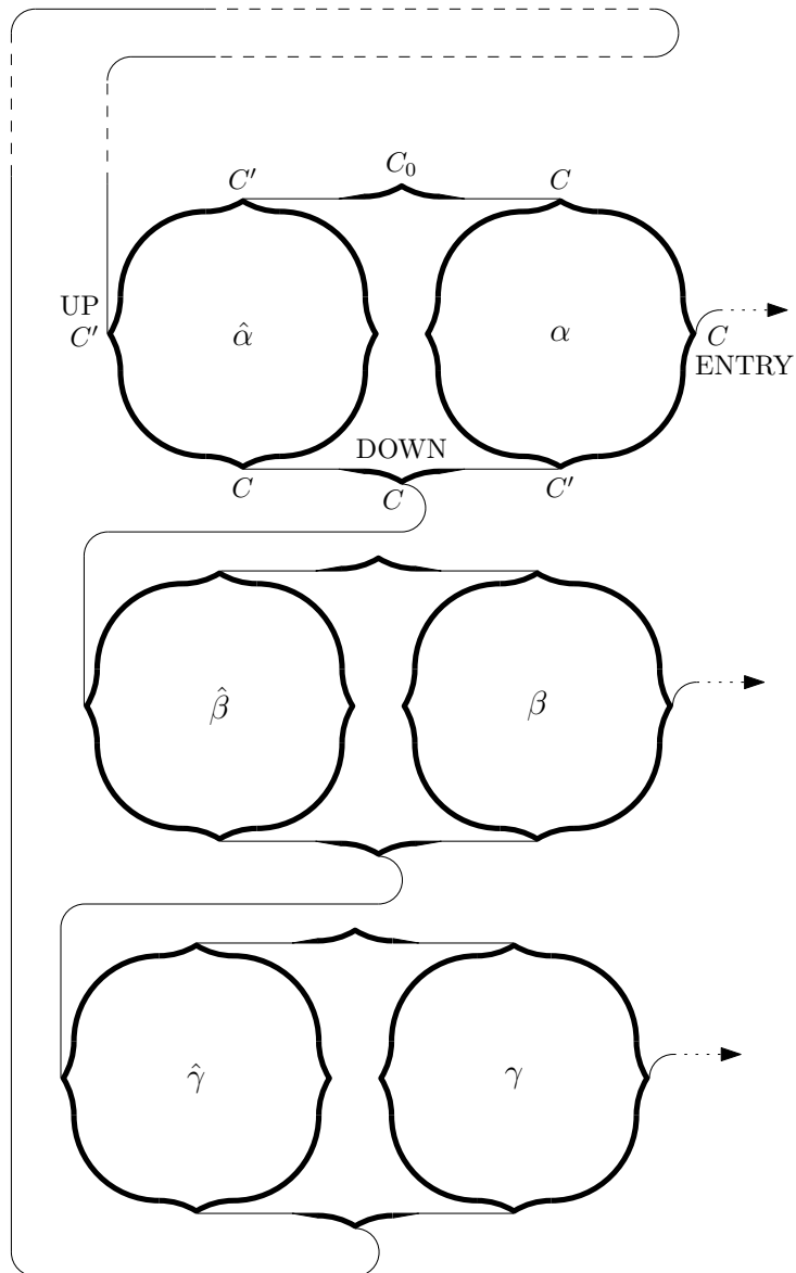
Fig. 21. Schematic view of the clause gadget. The dashed parts of the wires are long enough for sufficiently many copies of the wire-piece and the extended wire-piece to ensure that the wire can reach from the lowest C connection to the left C' connection of \hat{\alpha} (Lemma 6.1).
