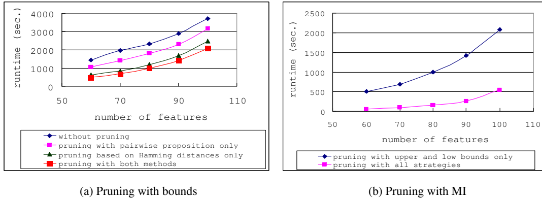
Figure 5: Pruning effects
