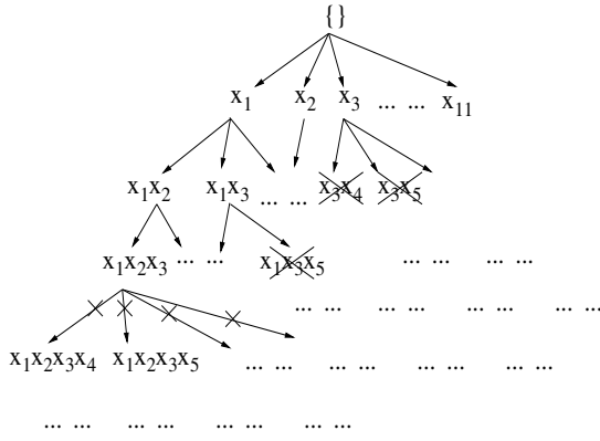
Figure 2: Enumerating candidate NIFSSs
