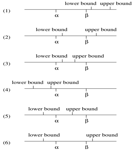
Figure 3: The possible relative positions of upper bound, lower bound, \alpha , and \beta
