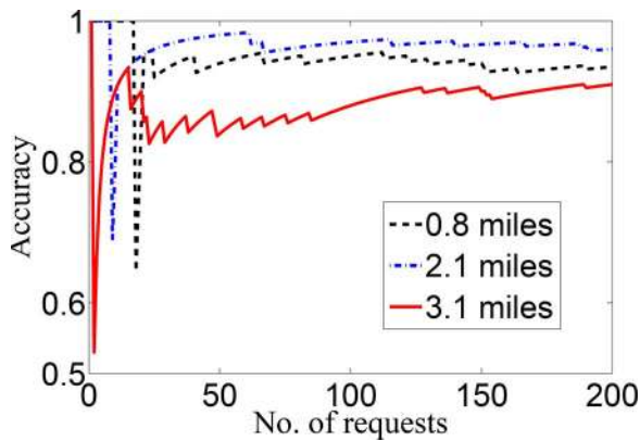
Fig. 8. Accuracy over time with different location contexts at 10am. ( \lambda = 50 mph).
