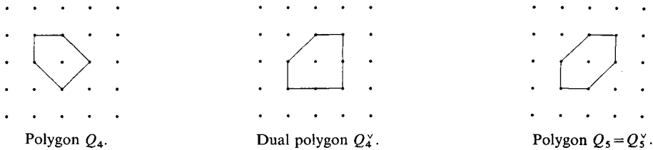
Polygon Q_5 = Q_5^v .
