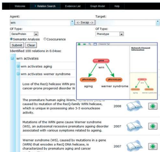
Figure 1. EXCERBT interface: (i) “which phenotypes are caused by the wrn gene?”; (ii) list of gene–phenotype pairs and detailed literature evidence; and (iii) graphical representation of selected relations.
