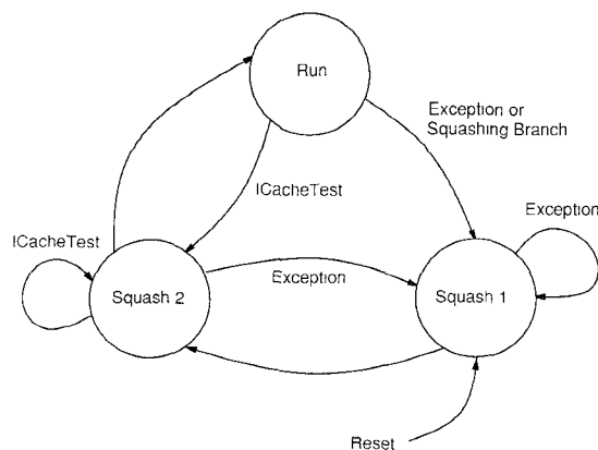
Fig. 13. Squash FSM.
