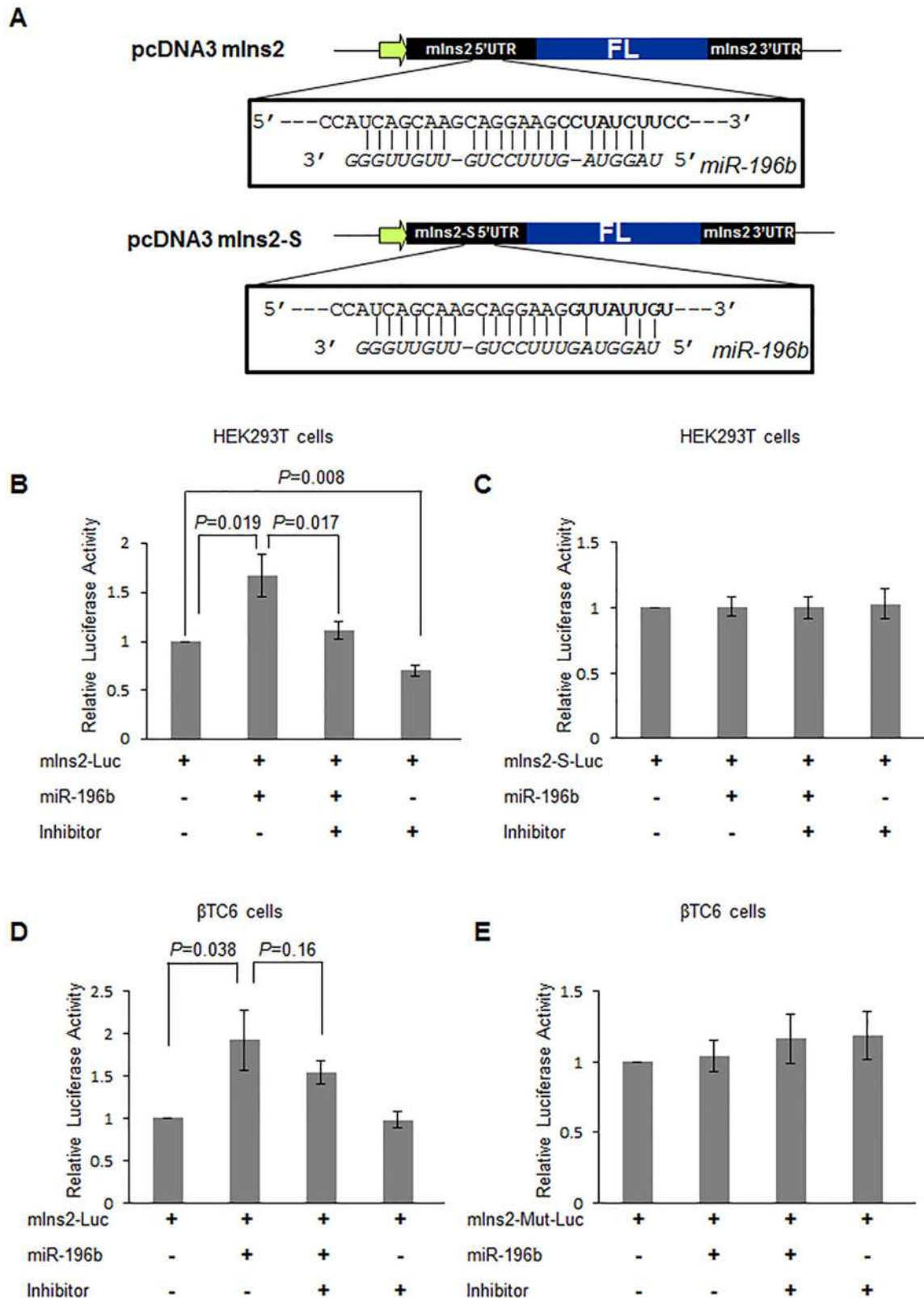
Figure 2. Translation activation mediated by miR-196b can be abolished by the anti miR-196b inhibitor. (A) Schematic representation of the reporter constructs for insulin2 and insulin2-S 5'UTR constructs. The bold letters in the RNA sequence represents the start of exon 2 of insulin2 mRNA and the lower italic letters represents the miR-196b sequence. The vertical lines between the sequences denote base pairing. (B, C) Anti-miR-196b was introduced into cells along with reporter and the miRNA-pSuper; 48 hr later, the effect of the miR-196b inhibitor was analyzed by measuring the relative luciferase activity in HEK293T cells transfected with insulin2 reporter (B) or insulin2-S reporter (C). (D, E) The miR-196b inhibitor and miR-196b duplex/control miRNA were introduced into \beta TC6 cells before transfecting with insulin2-luciferase reporter (D) or the mutant-reporter
