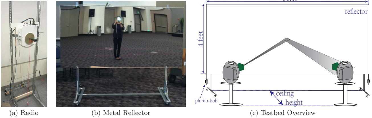
Figure 4: Our 3D beamforming testbed. (a) The 60GHz radio with horn antenna, mounted on top of a mobile platform with adjustable height. (b) A 4ft×8ft, mirror-quality stainless steel reflector mounted vertically on a mobile platform. (c) An illustration of the experiment configuration.
