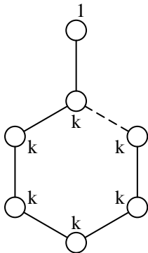
Figure 1: Quiver diagram for the B-model of U(k) gauge theory
