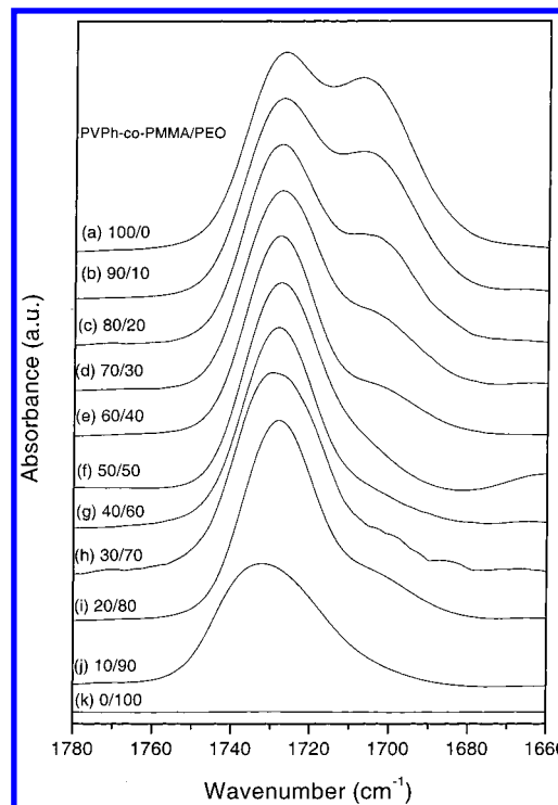
Figure 6. FTIR spectra recorded at room temperature in the 1660–1780 \text{cm}^{-1} region for PVPh-co-PMMA/PEO blends: (a) 100/0; (b) 90/10; (c) 80/20; (d) 70/30; (e) 60/40; (f) 50/50; (g) 40/60; (h) 30/70; (i) 20/80; (j) 10/90; (k) 0/100.
