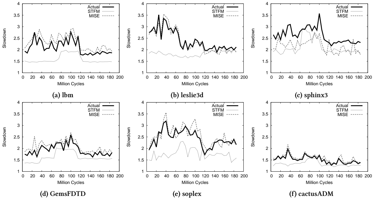
Figure 2: Comparison of our MISE model with STFMs for representative memory-bound applications
