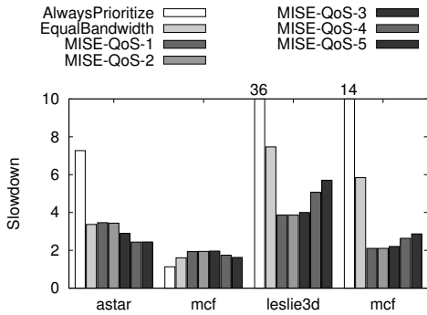
Figure 7: Meeting a target bound for two applications
