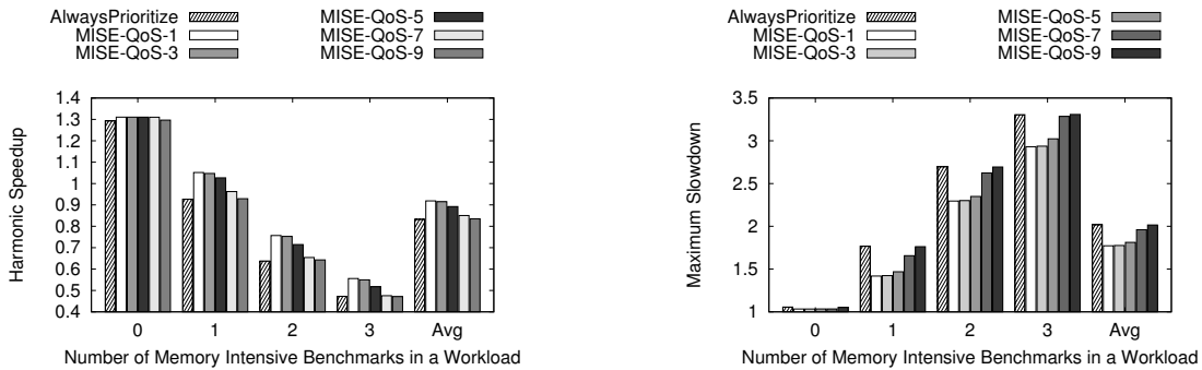
Figure 5: Average system performance and fairness across 300 workloads of different memory intensities
