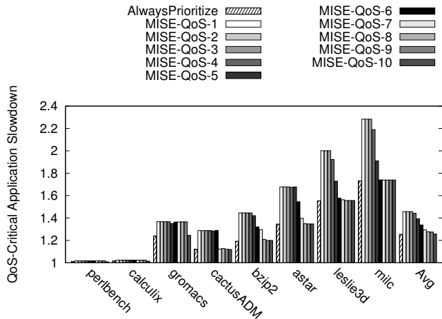
Figure 4: AoI performance: MISE-QoS vs. AlwaysPrioritize
