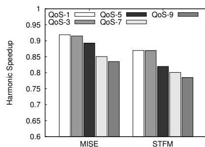
Figure 6: Average system performance using MISE and STFMs’s slowdown estimation models (across 300 workloads)
