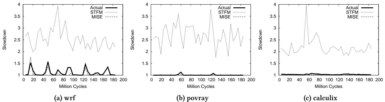
Figure 3: Comparison of our MISE model with STFMs for representative non-memory-bound applications
