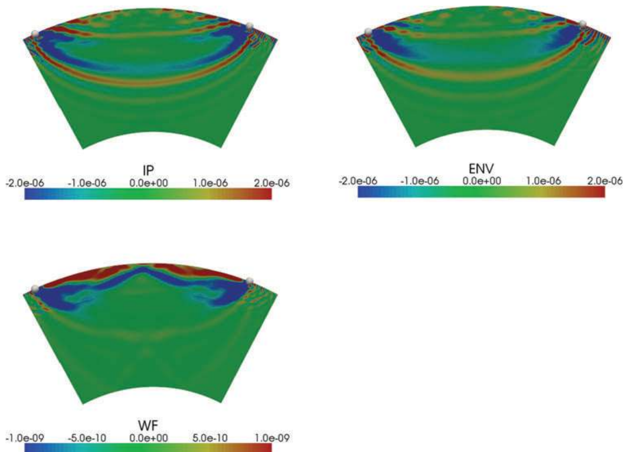
Figure 15. Source–receiver cross-sections of K_\beta adjoint kernels for complete seismograms computed based on the adjoint sources shown in Fig. 14.
