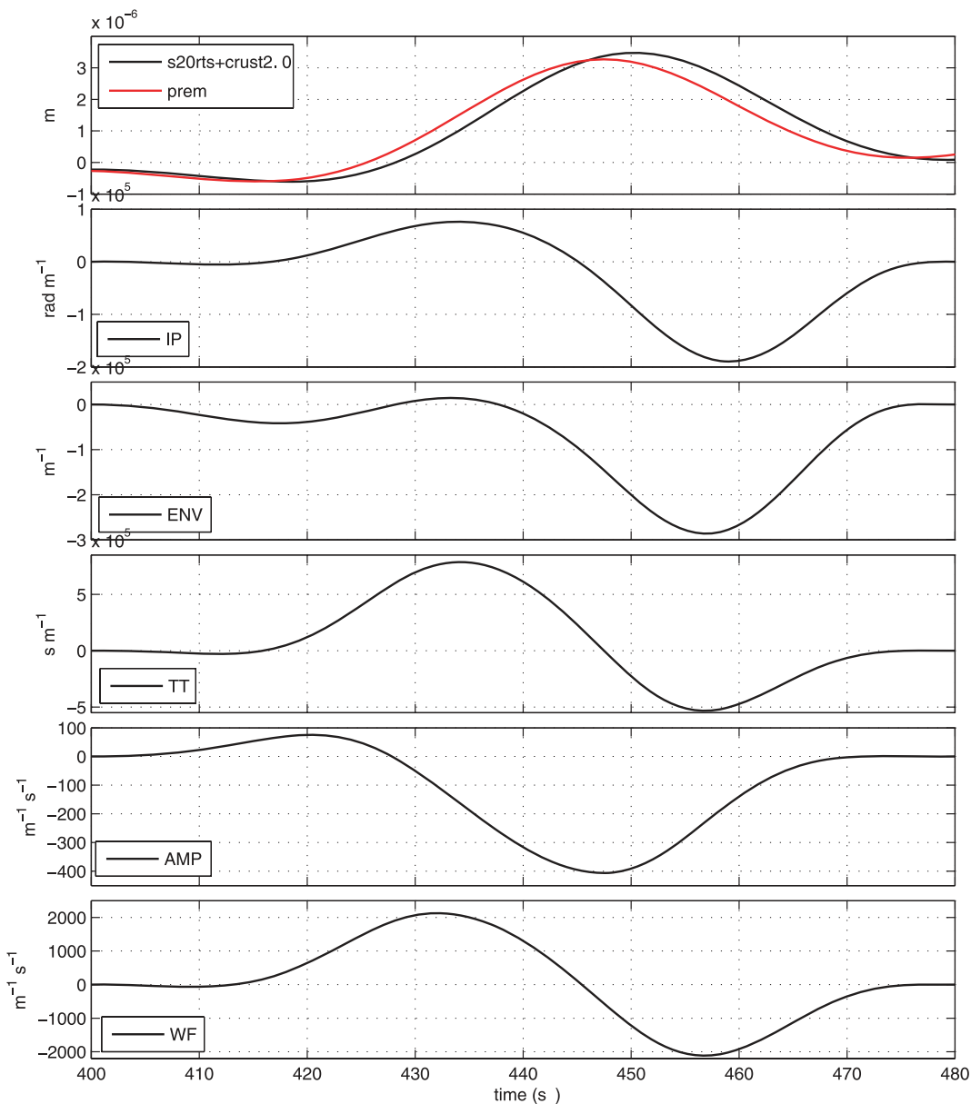
Figure 5. Adjoint sources for the first arriving P wave (top) cut from seismograms in Fig. 3 using IP, ENV, TT, AMP and normalized WF measurements. Adjoint sources are computed for full seismograms, then a cosine taper is applied to extract the adjoint source for the time window of the phase of interest.
