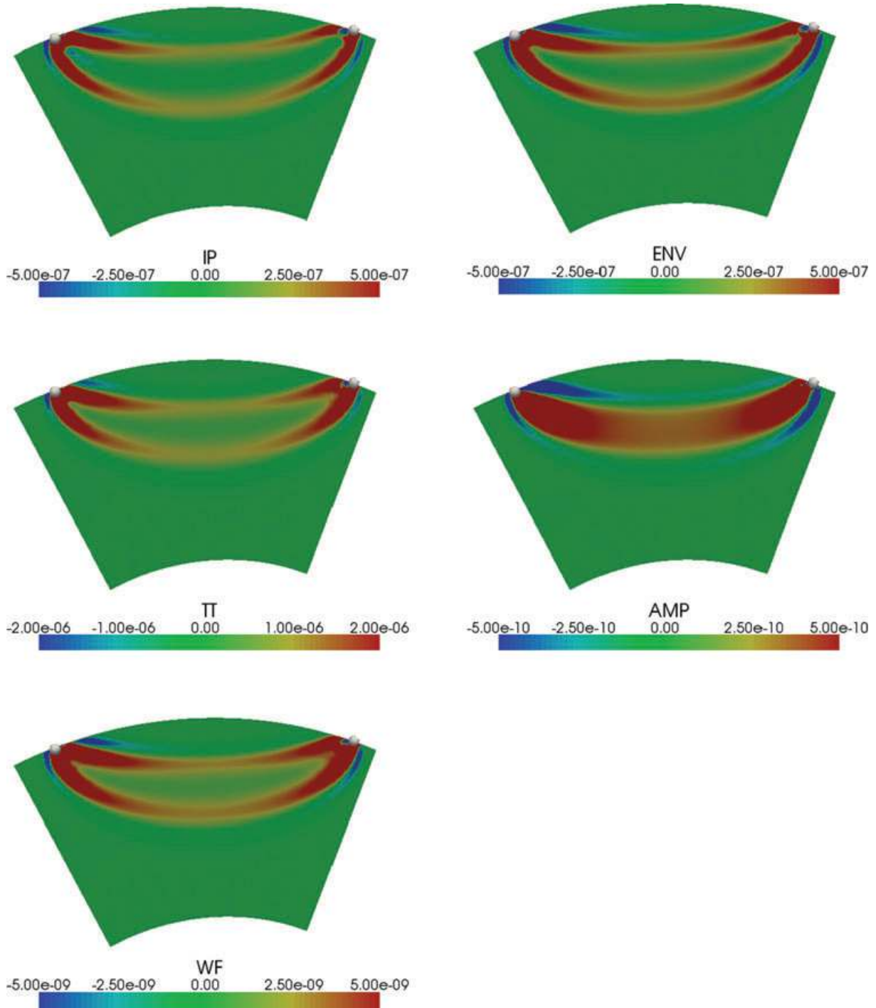
Figure 6. Source–receiver cross-sections of K_\alpha adjoint kernels for P waves computed based on the adjoint sources in Fig. 5. Units of the kernels are \text{rad s}^{-3} for instantaneous phase misfit (IP), \text{s m}^{-3} for envelope misfit, \text{s}^2 \text{m}^{-3} for travelt ime misfit (TT), \text{m}^{-3} for amplitude misfit (AMP), \text{m}^{-3} for normalized waveform misfit (WF).
