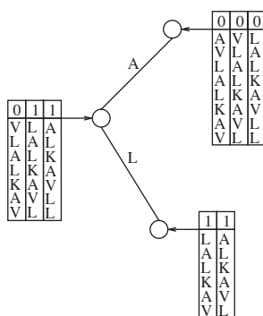
Fig. 2. An (8, 1) -mismatch tree for a sequence AVLALKAVLL used for computing the kernel matrix with k -mers of length 8 allowing 1 mismatch. The path from the root to the node is the ‘prefix’ of a particular k -mer feature. The leaf node stores the number of mismatches between the prefix of a k -mer instance and the prefix of a feature and a pointer to the tail of the k -mer. The figure shows the tree after expanding the path AL.
