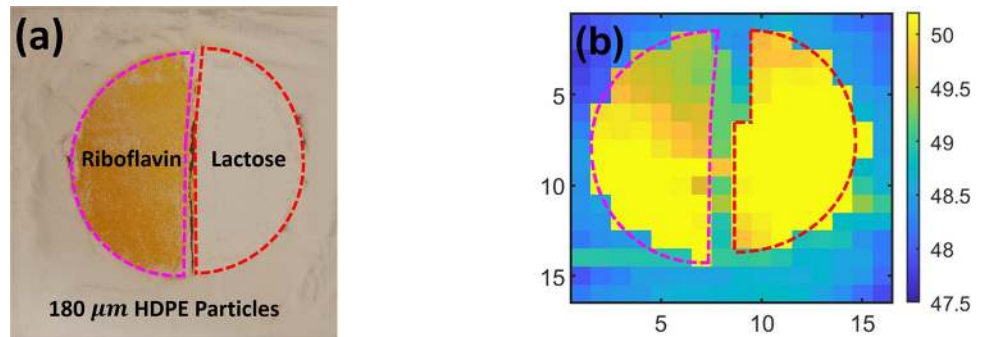
Fig 6. Visual and time-of-arrival image. (a) The visual image of the pellet that was buried beneath 2 mm of 180 \mu\text{m} HDPE particles is shown with dashed outlines for lactose (red) and riboflavin (magenta). (b) The time-of-arrival image of the pellet at \theta_0 is also shown with outlines for each pellet material.
