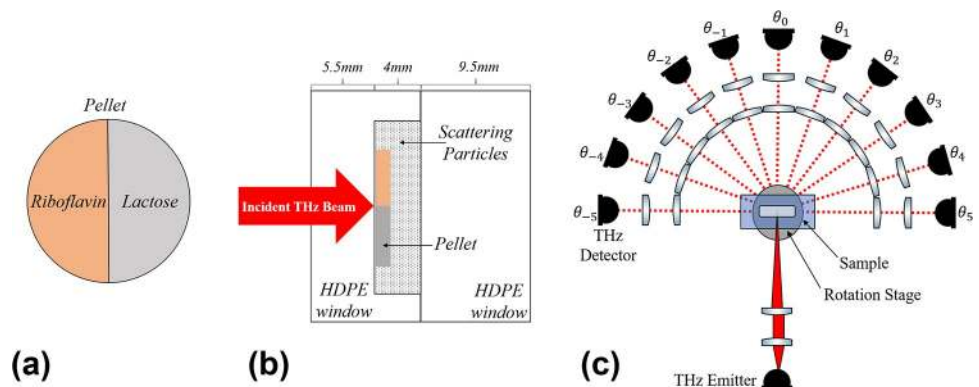
Fig 1. Sample and experimental setup. (a) The pellet with two different materials with unique spectral peaks in the THz regime is shown. (b) The sample location is shown in a cross-section of the sample holder which is made from two HDPE slabs. (c) The optical setup used for measuring diffused granular scattering signal is depicted. The THz detector arm was on a rotation stage and measurement angles, \theta_{\pm n} , were in steps of 18°.
