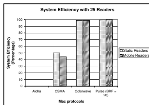
Fig. 8. Efficiency with 25 Readers
