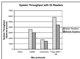
Fig. 7. Throughput comparison with 25 readers
