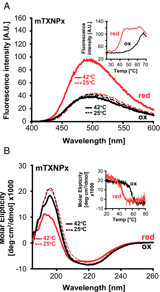
Fig. 4. mTXNPx undergoes temperature-mediated structural changes. (A) Bis-ANS binding to mTXNPx red (red lines) or mTXNPx ox (black lines) at either 25 °C (broken lines) or 42 °C (solid lines). (Inset) Bis-ANS binding of mTXNPx red or mTXNPx ox as a function of temperature monitored at 500 nm. (B) Far-UV circular dichroism spectra of mTXNPx red (red lines) or mTXNPx ox (black lines) at either 25 °C (dashed lines) or 42 °C (solid lines). (Inset) Temperature-dependent changes in the secondary structure of mTXNPx red or mTXNPx ox recorded at 197 nm. Temperature was increased at a rate of 1 °C/min. All spectra were buffer corrected.
